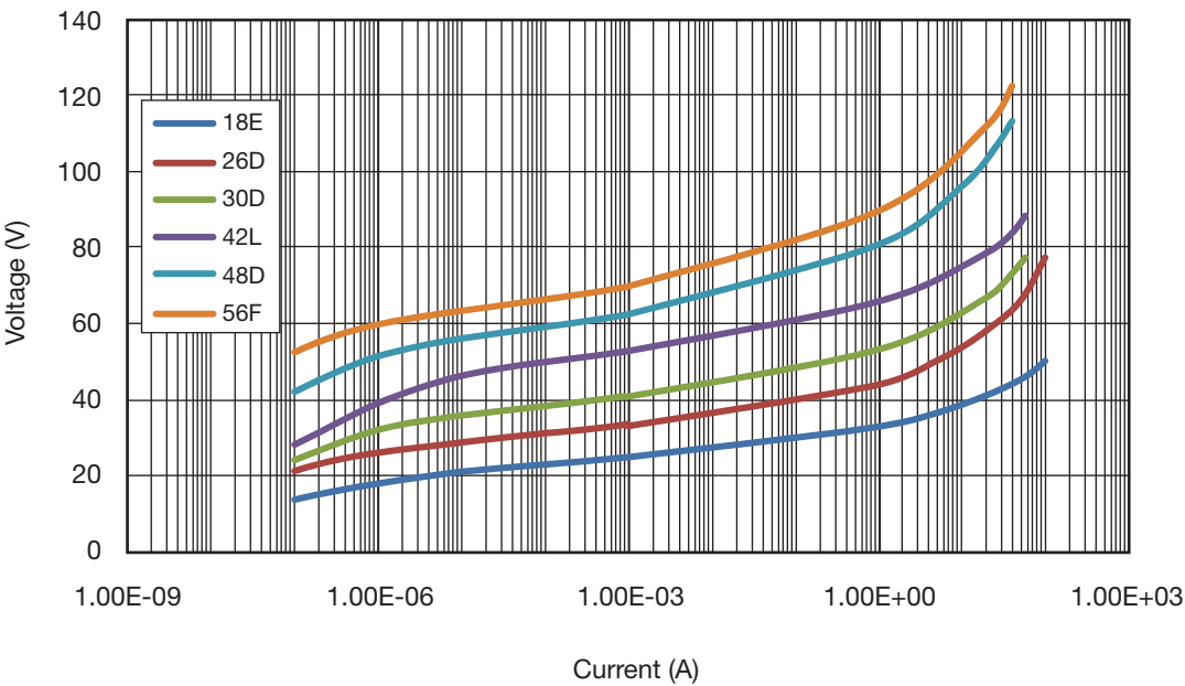
1206 Case Size
