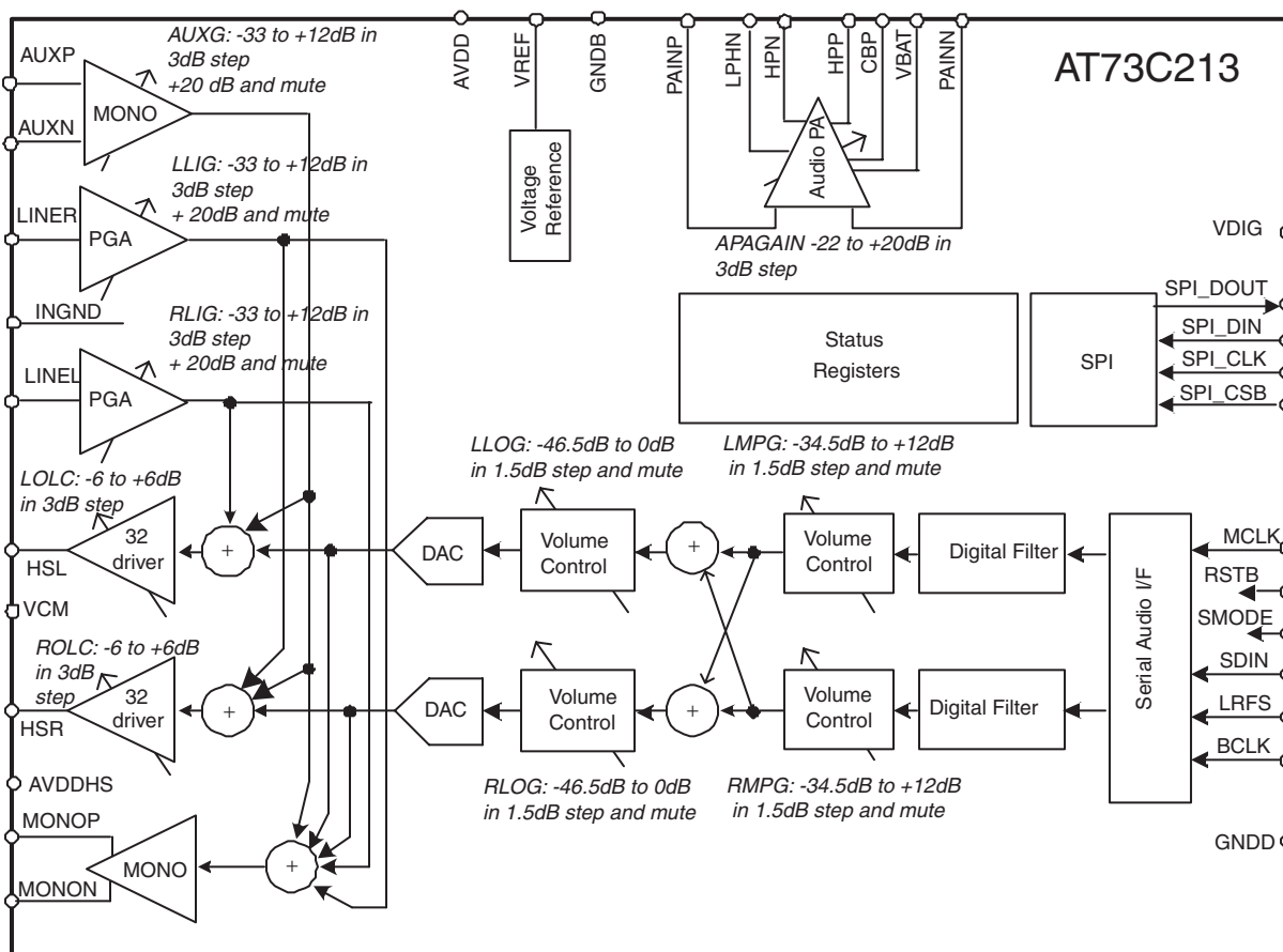
Figure 2-1. AT73C213 Functional Block Diagram
