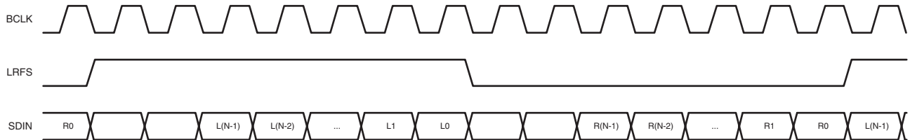
Figure 7-6. 20-bit LSB Justified Mode
