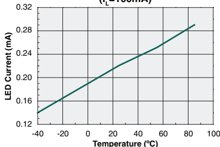
Form-B Typical I_F for Switch Operation vs. Temperature ( I_L=100mA )
