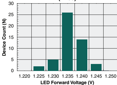
Form-B Typical LED Forward Voltage Drop (N=50)
