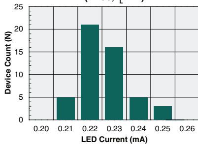
Form-B Typical LED Current to Operate (N=50, I_L=1A )
