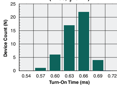
Form-B Typical Turn-On Time (N=50, I_F=5mA )
