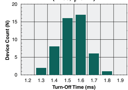
Form-B Typical Turn-Off Time (N=50, I_F=5mA )
