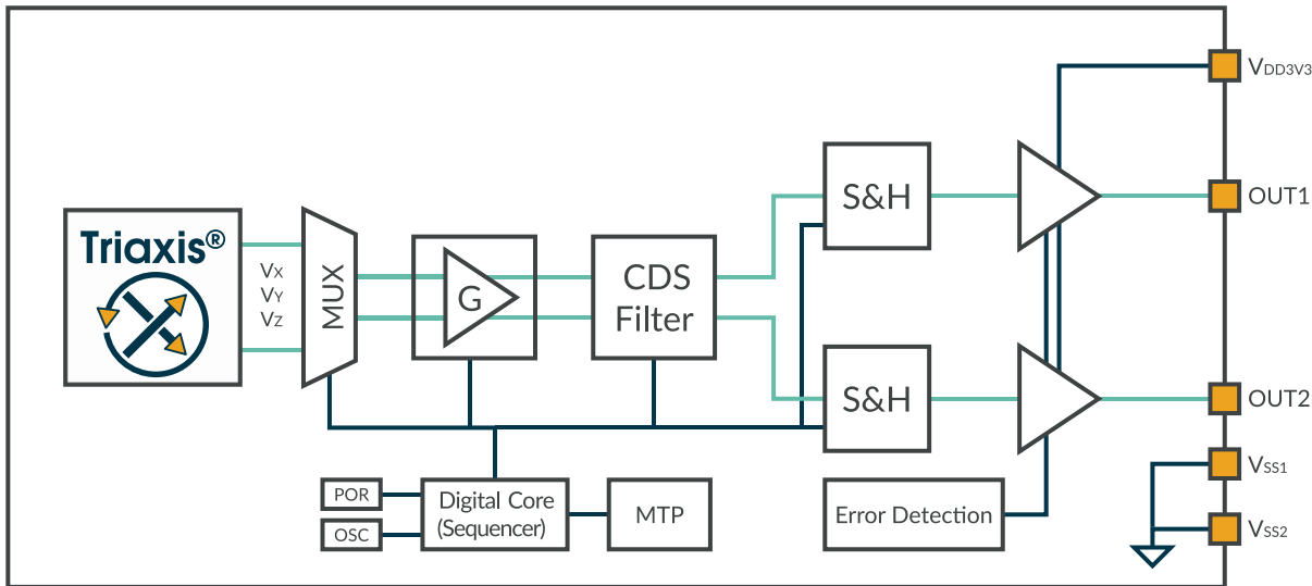
Figure 1 – Functional diagram
