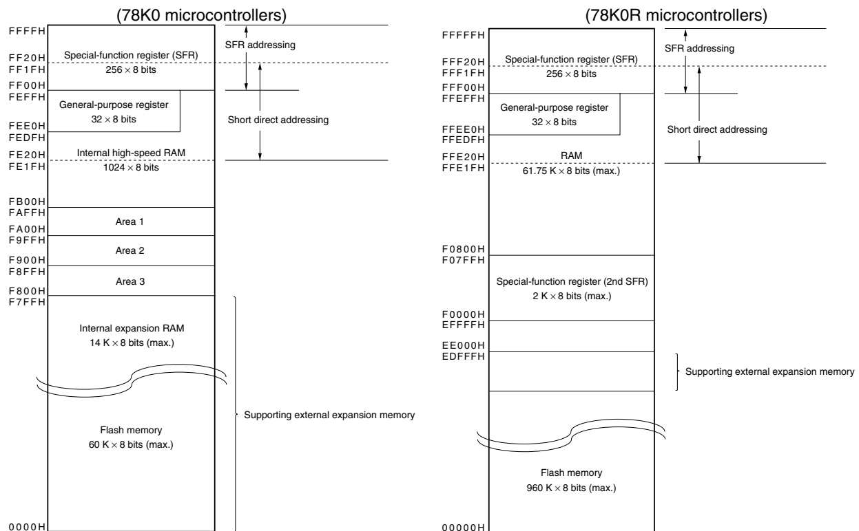
Figure 2-1. Memory Maps of 78K0 Microcontrollers and 78K0R Microcontrollers
