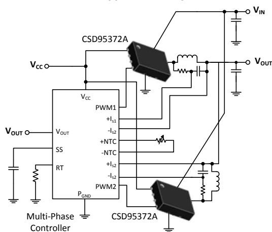
Application Diagram
