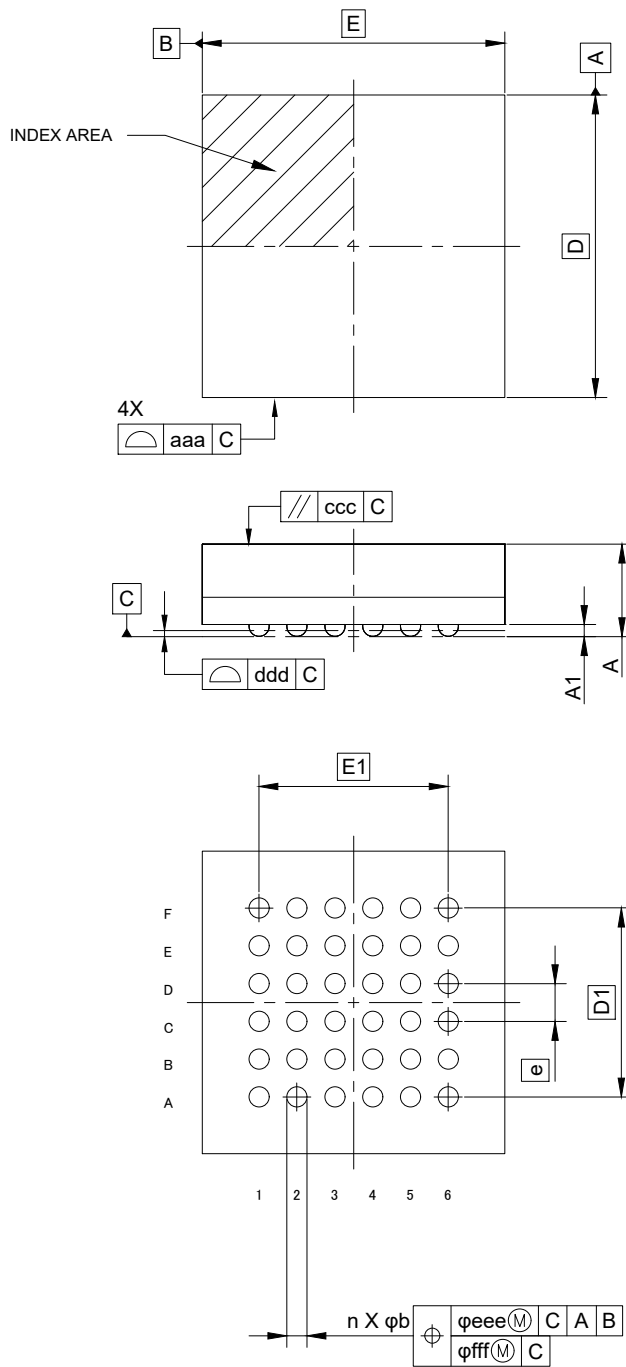
Figure A2.5 BGA 36-pin
