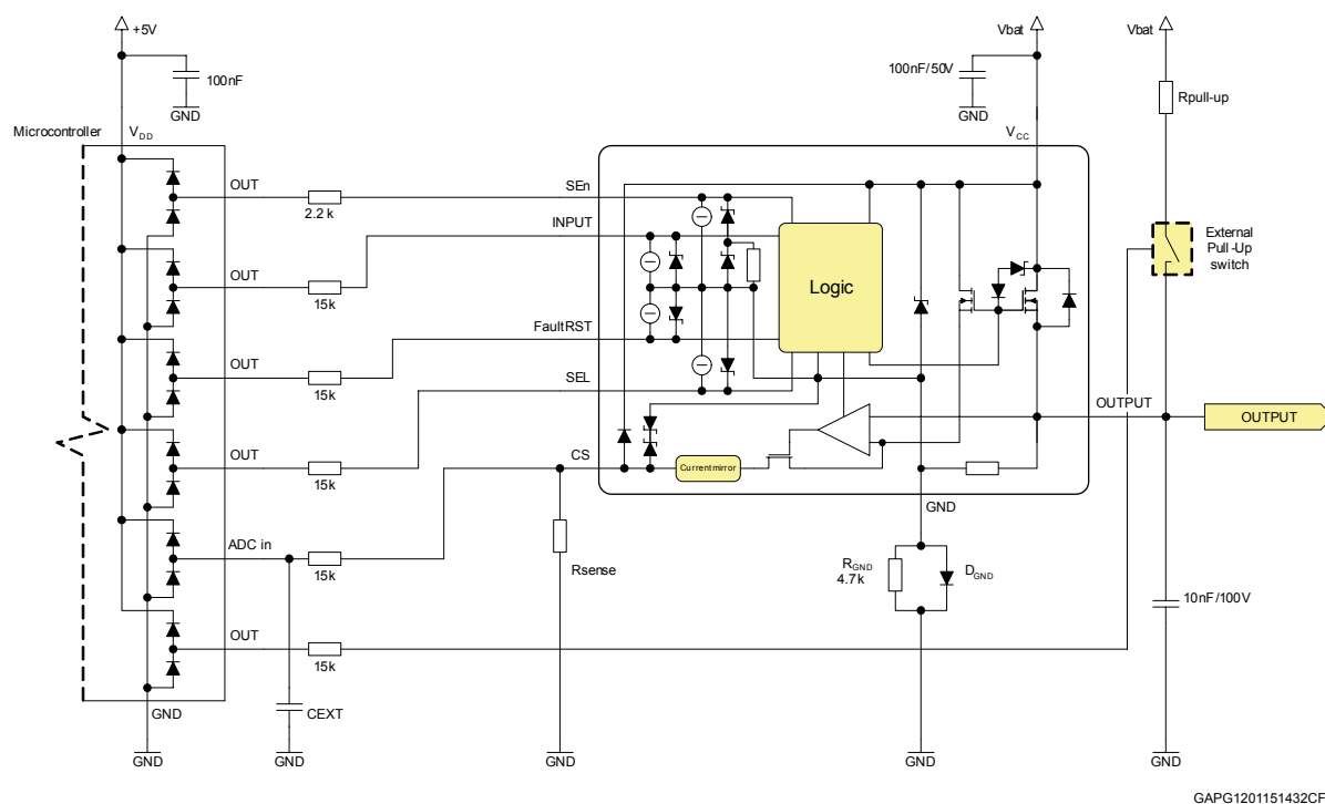
Figure 38. Open-load / short to V_{CC} condition
