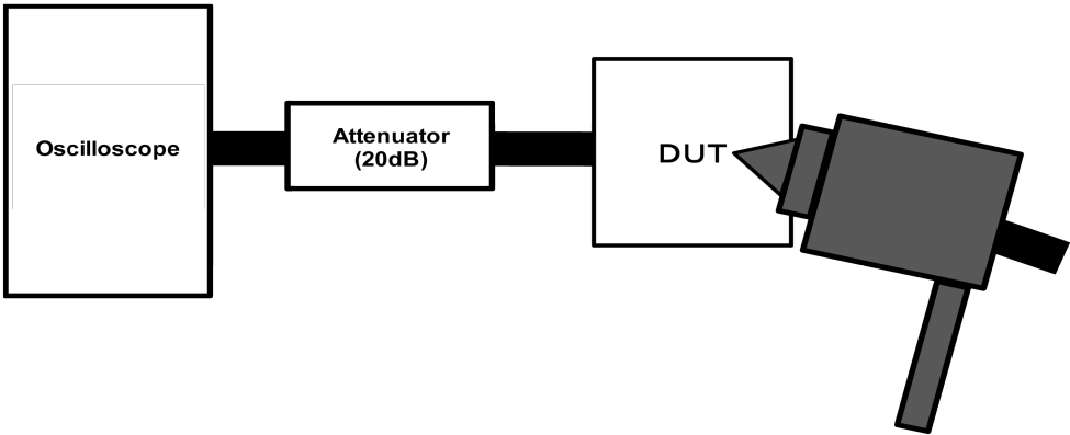
Fig. 11.3 IEC61000-4-2 (Contact)
