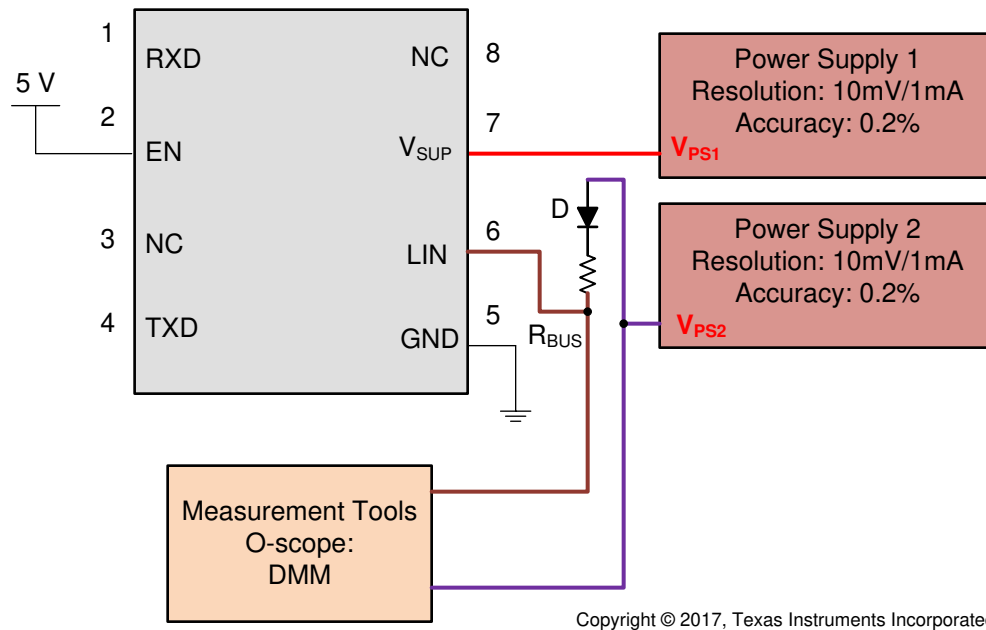
Figure 8-5. V<sub>SUP</sub>_NON_OP Param 11
