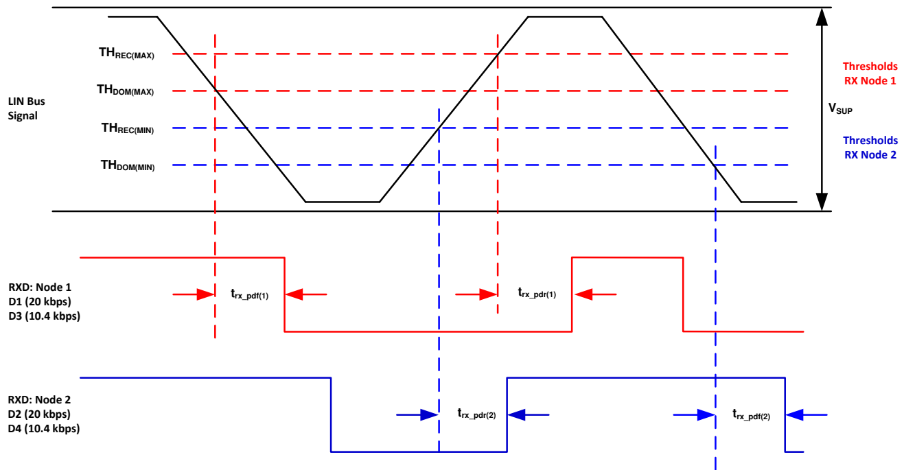
Figure 8-14. Propagation Delay
