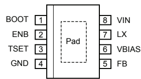
Pin Out Diagram
