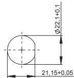
Drilling diagram
