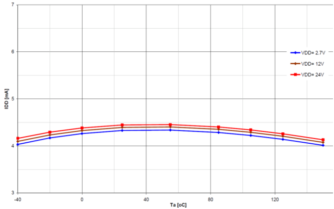
10.5. I_{DD} vs. T_A
