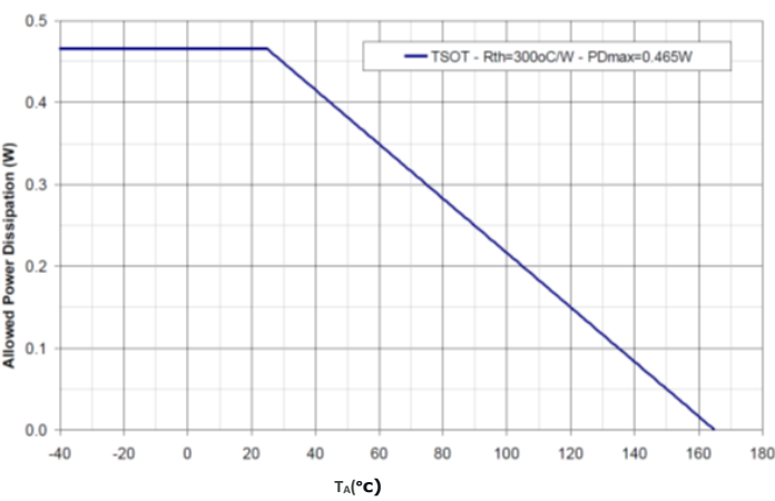
10.9. Power Derating vs. T_A
