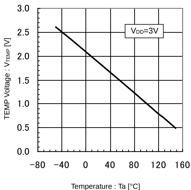
Figure 1. TEMP Voltage vs Temperature (Temperature Sensitivity)
