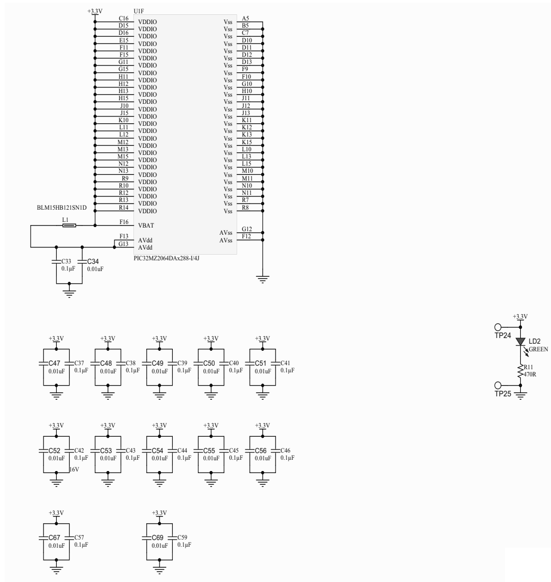
FIGURE A-4: PIC32MZ2064DAX288 DAUGHTER CARD SCHEMATICS (4 OF 4)
