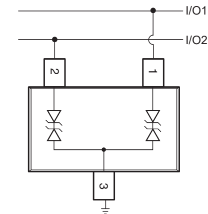
Bidirection Protection of Two Lines
