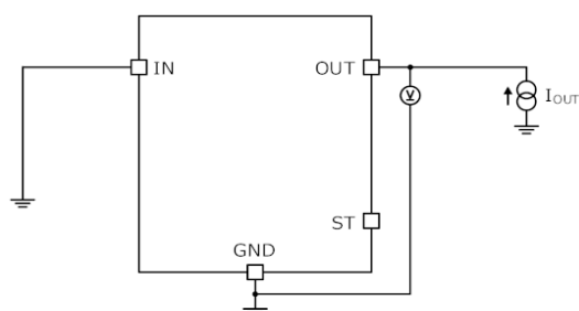
Measurement Circuit for Figure 8, Figure 9
