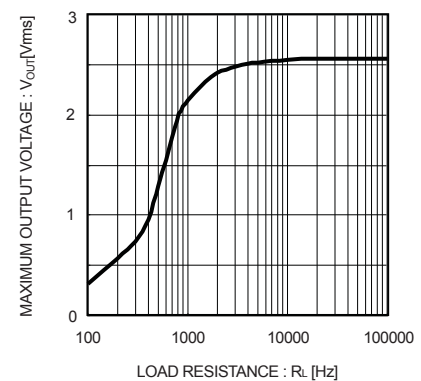
Fig.11 Output load characteristic (BD3822FS, BD3824FS)
