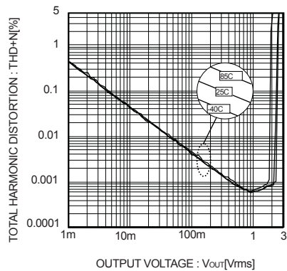
Fig.5 Total harmonic distortion vs Output voltage (BD3822FS)
