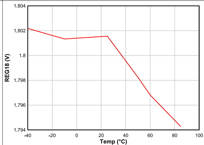
Figure 7-25. REG18 Voltage vs. Temperature, with No Load
