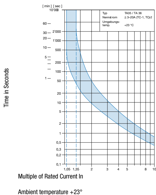
Tripping Characteristics thermal I_n \geq 3 \dots \leq 20A
