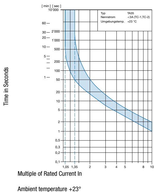
Tripping Characteristics thermal I_n < 3A
