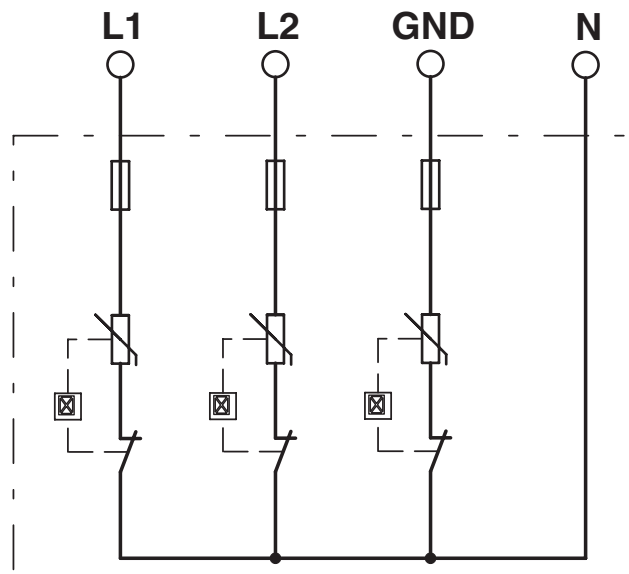
Circuit diagram
