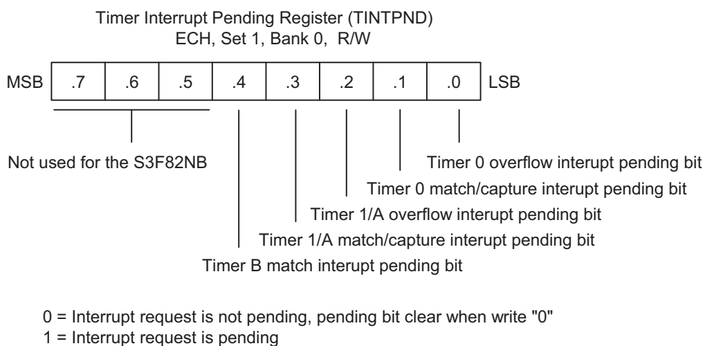
Figure 12-3. Timer Interrupt Pending Register (TINTPND)
