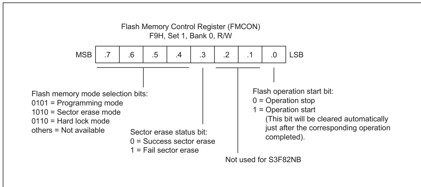
Figure 18-1. Flash Memory Control Register (FMCON)
