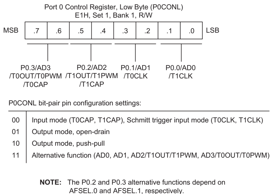
Figure 9-3. Port 0 Low-Byte Control Register (P0CONL)
