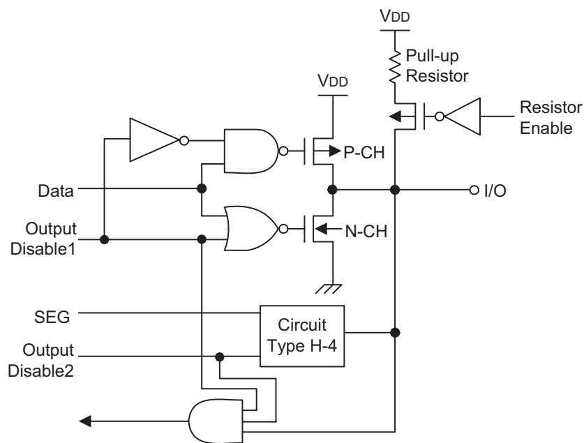
Figure 1-13. Pin Circuit Type H-10 (P7-P10)
