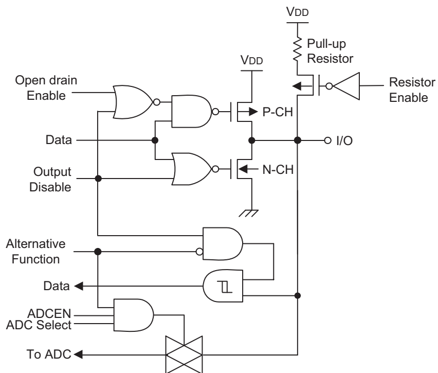
Figure 1-9. Pin Circuit Type F-4 (P0.0 – P0.1) PRELIMINARY
