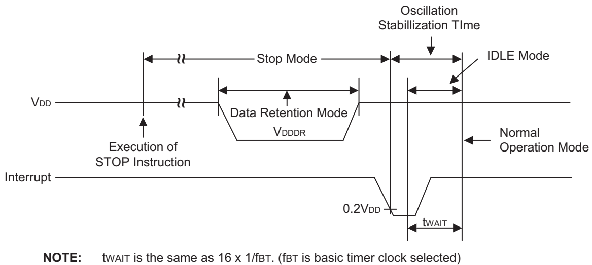
Figure 19-4. Stop Mode Release Timing Initiated by Interrupts
