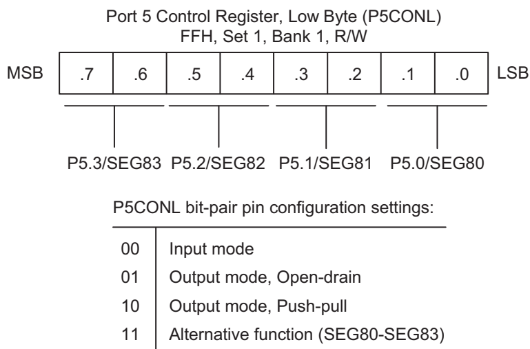
Figure 9-22. Port 5 Low-Byte Control Register (P5CONL)
