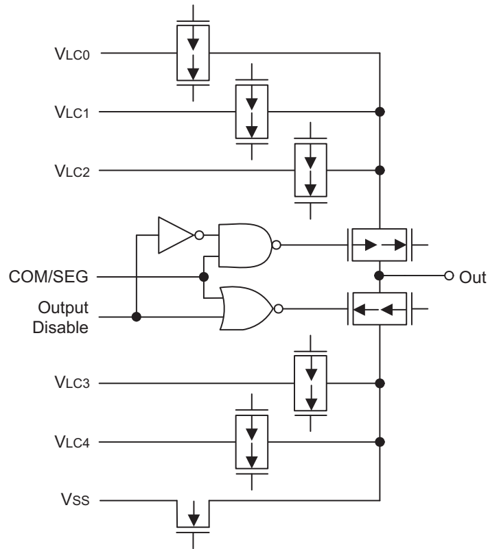
Figure 1-10. Pin Circuit Type H-4
