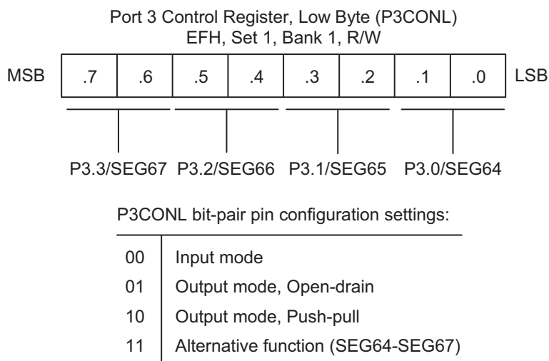
Figure 9-16. Port 3 Low-Byte Control Register (P3CONL)
