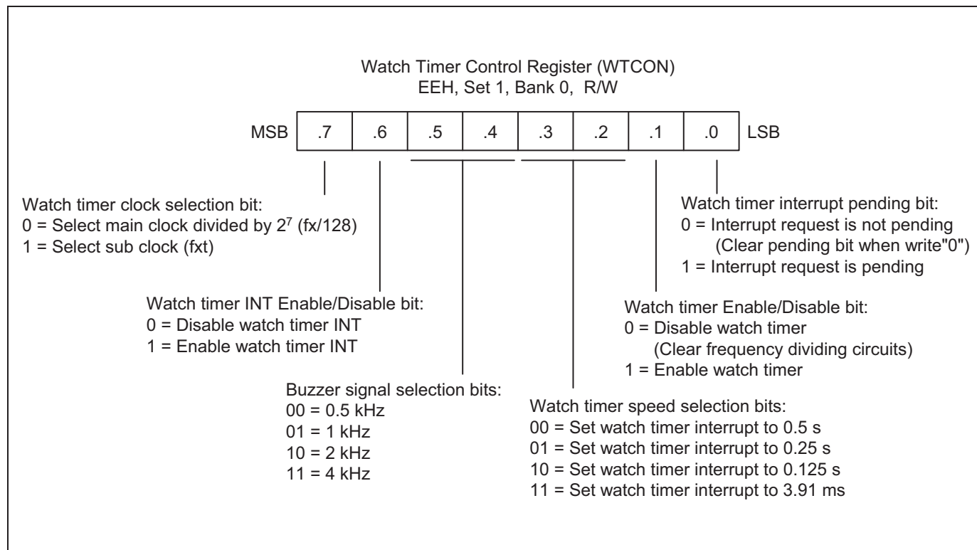
Figure 13-1. Watch Timer Control Register (WTCN)
