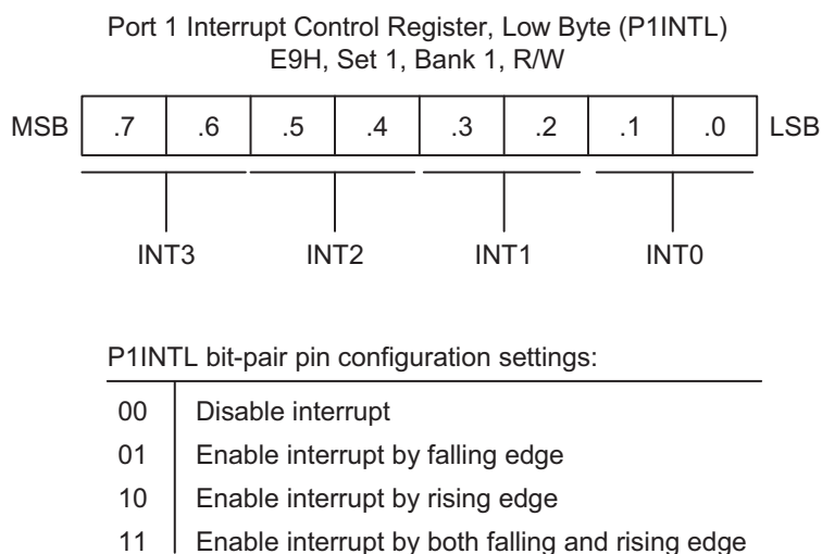
Figure 9-10. Port 1 Low-Byte Interrupt Control Register (P1INTL)
