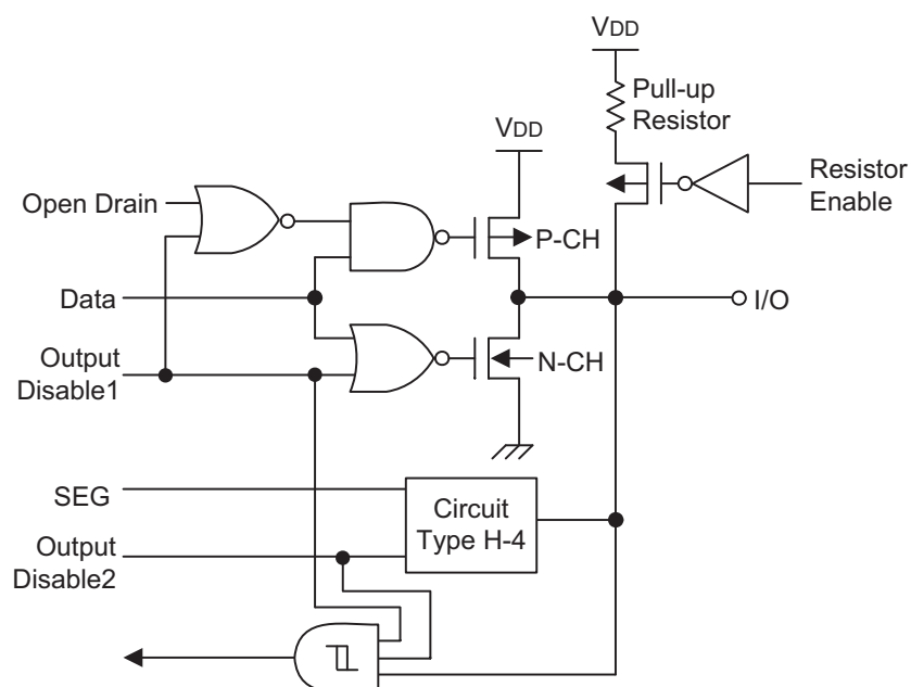
Figure 1-12. Pin Circuit Type H-9 (P5.4-P5.7)
