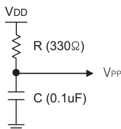
Figure 21-2. RC Delay Circuit
