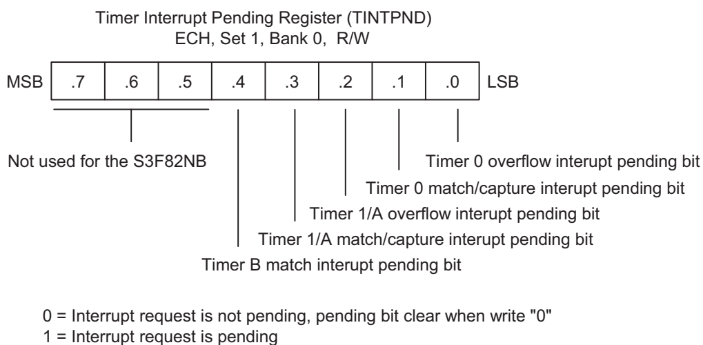
Figure 12-10. Timer Interrupt Pending Register (TINTPND)
