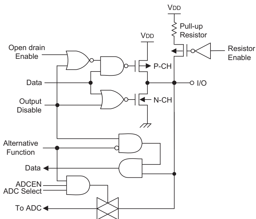
Figure 1-6. Pin Circuit Type F-3 (P0.2-P0.7)
