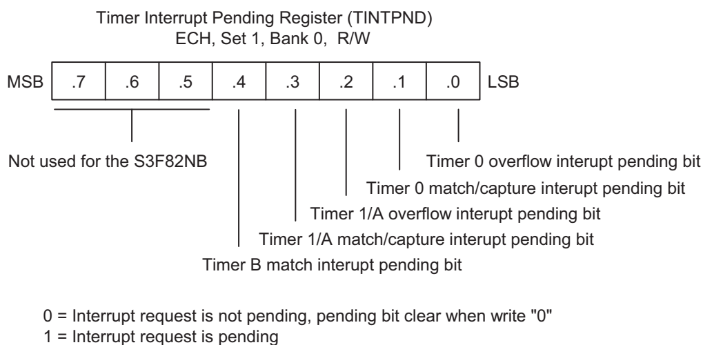
Figure 12-17. Timer Interrupt Pending Register (TINTPND)
