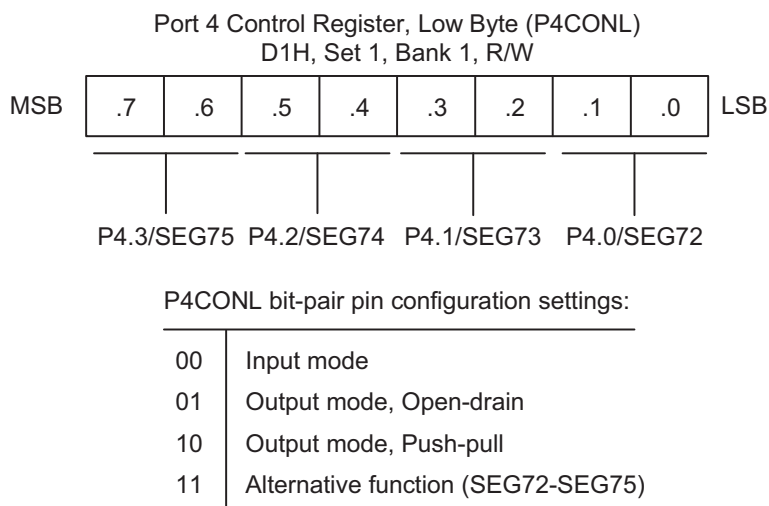
Figure 9-19. Port 4 Low-Byte Control Register (P4CONL)
