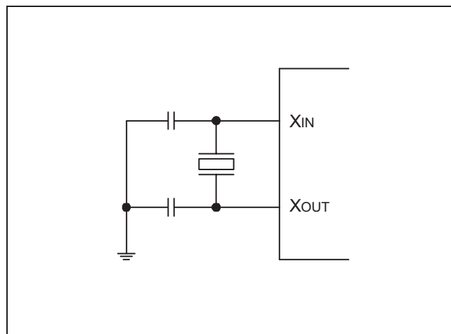
Figure 7-1. Crystal/Ceramic Oscillator (fx)
