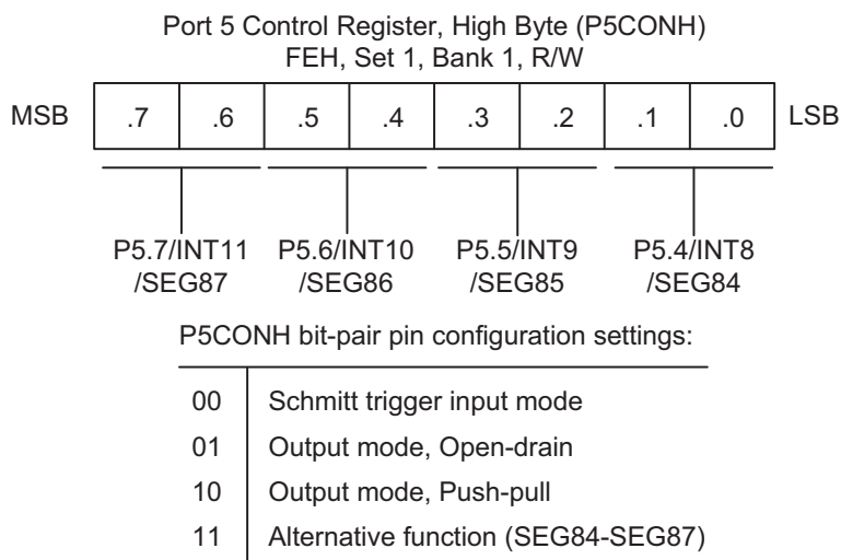
Figure 9-21. Port 5 High-Byte Control Register (P5CONH)
