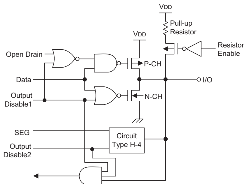
Figure 1-11. Pin Circuit Type H-8 (P2-P4, P5.0-P5.3)
