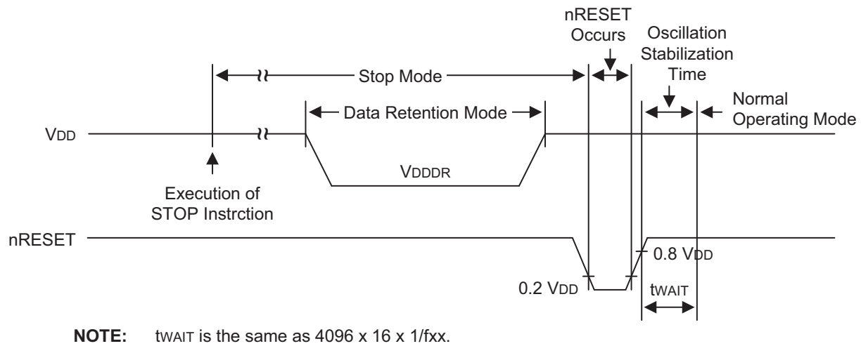
Figure 19-3. Stop Mode Release Timing Initiated by nRESET
