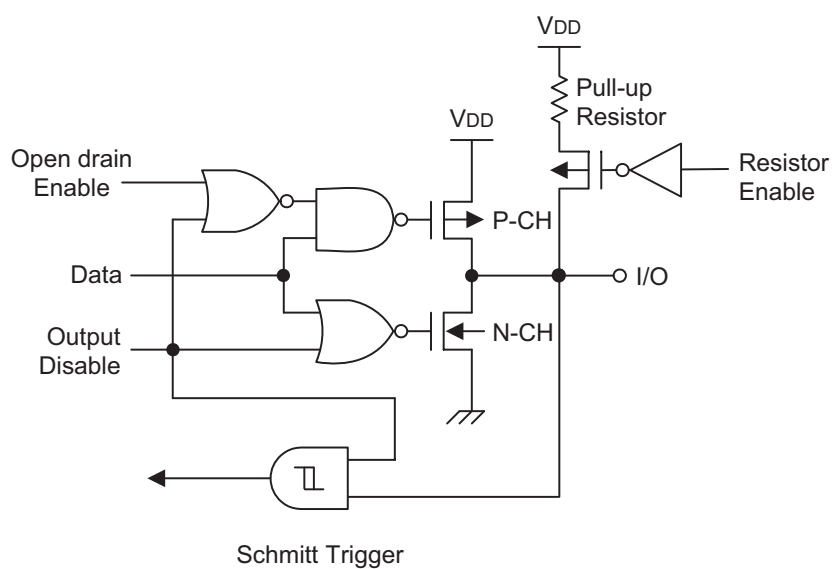
Figure 1-7. Pin Circuit Type E-4 (P1 except P1.0)
