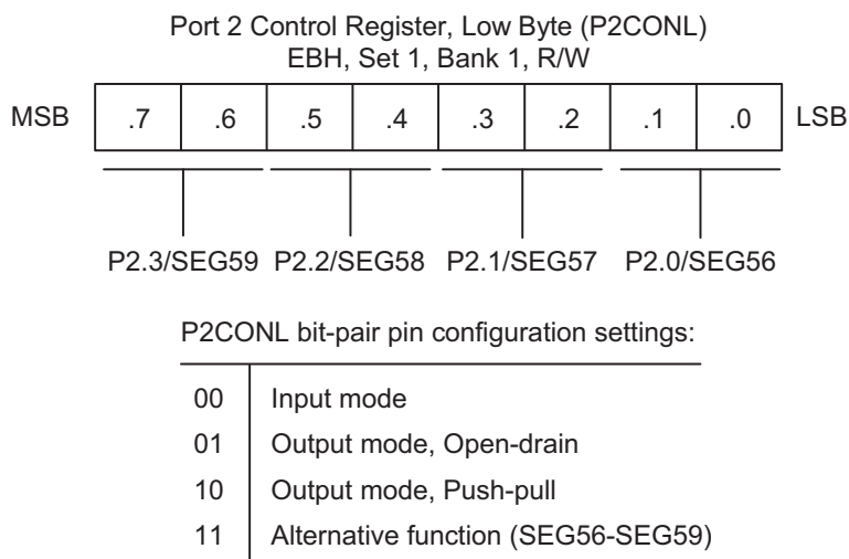
Figure 9-13. Port 2 Low-Byte Control Register (P2CONL)
