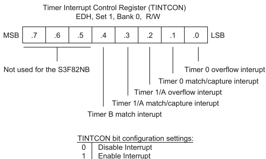
Figure 12-2. Timer Interrupt Control Register (TINTCON)
