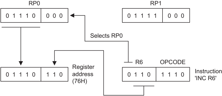
Figure 2-13. 4-Bit Working Register Addressing Example
