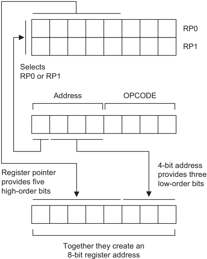
Figure 2-12. 4-Bit Working Register Addressing
