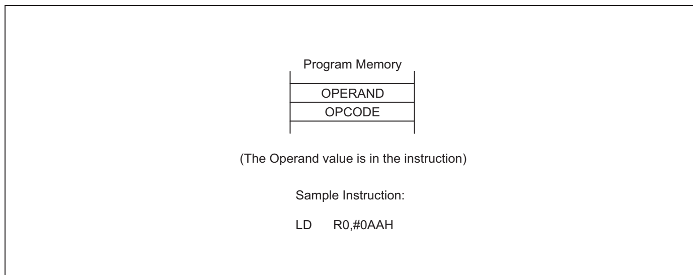
Figure 3-14. Immediate Addressing
