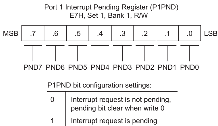
Figure 9-11. Port 1 Interrupt Pending Register (P1PND)
