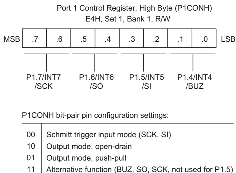
Figure 9-6. Port 1 High-Byte Control Register (P1CONH)
