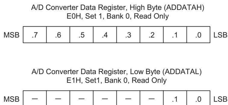
Figure 15-2. A/D Converter Data Register (ADDATAH/L)
