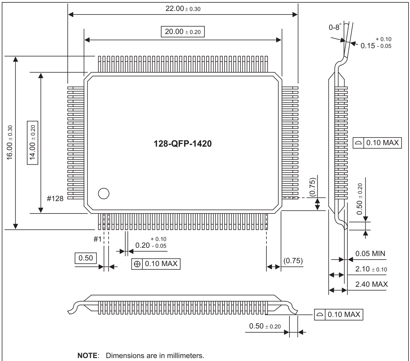
Figure 20-1. Package Dimensions (128-QFP-1420) PRELIMINARY
