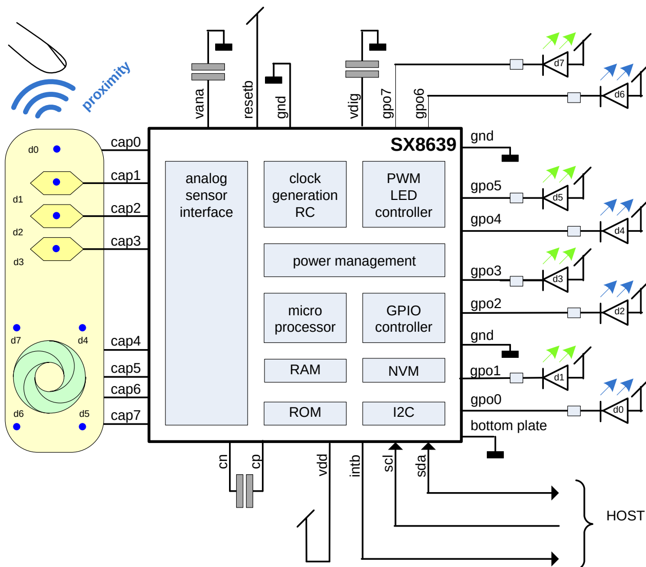
Figure 61 Typical Application
