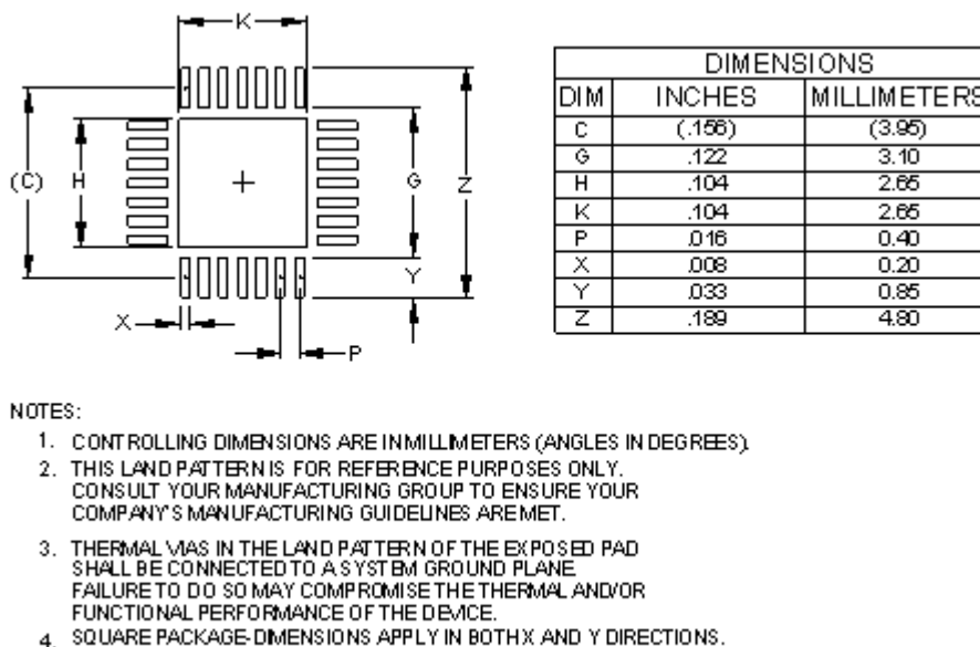
Figure 70 Land Pattern
