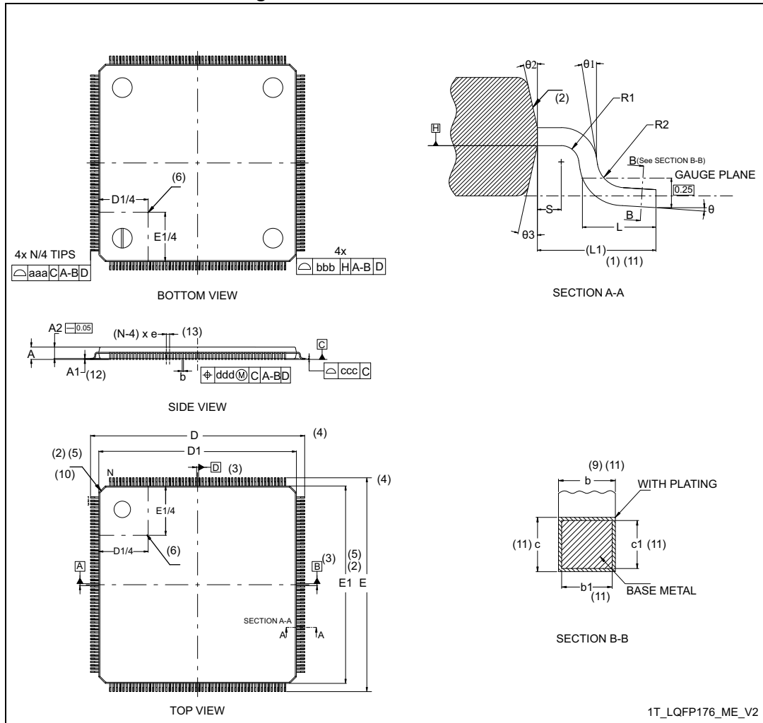
Figure 127. LQFP176 - Outline (15)
