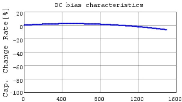
DE1B3RA101KJ4BQ01F C-DC bias capchange, 20.0
