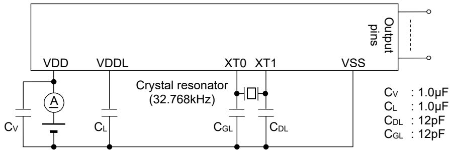
Measuring circuit 2
