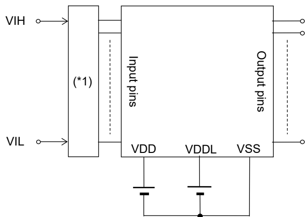
Measuring circuit 5
