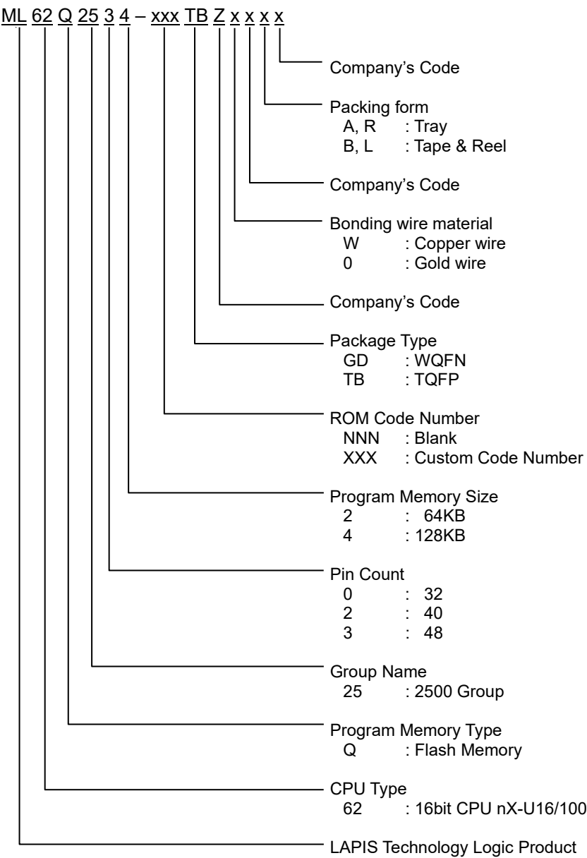
Figure 1 Part Number
