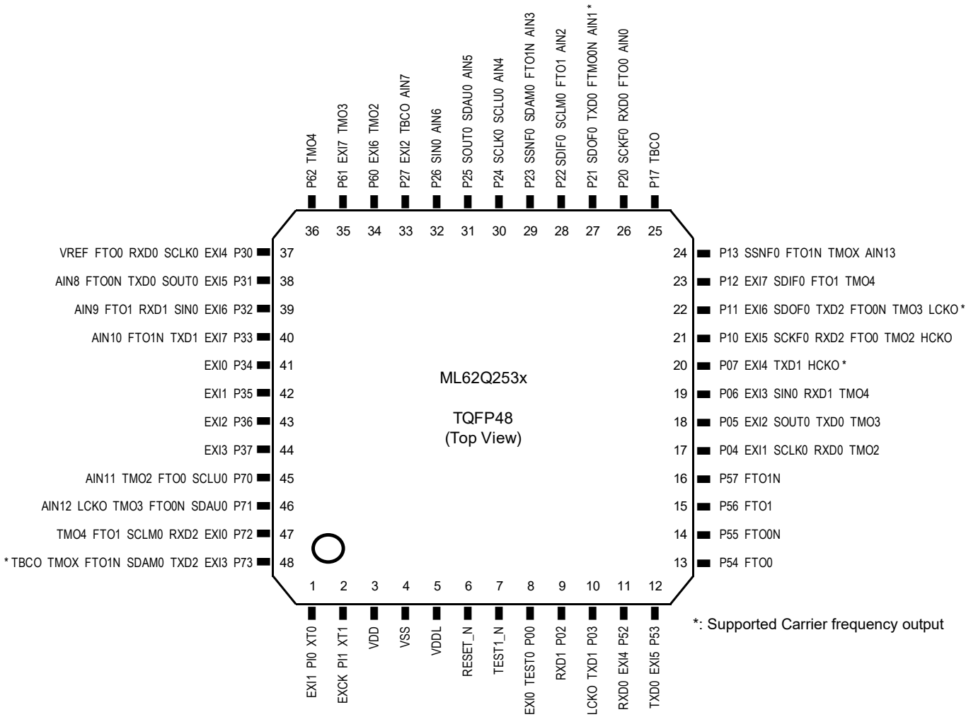
Fig.3-1 48 pin TQFP
