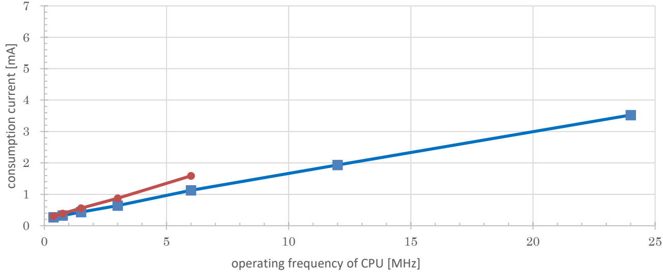
(1) PLL 24MHz (TYP.)
