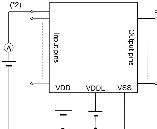
Measuring circuit 4
