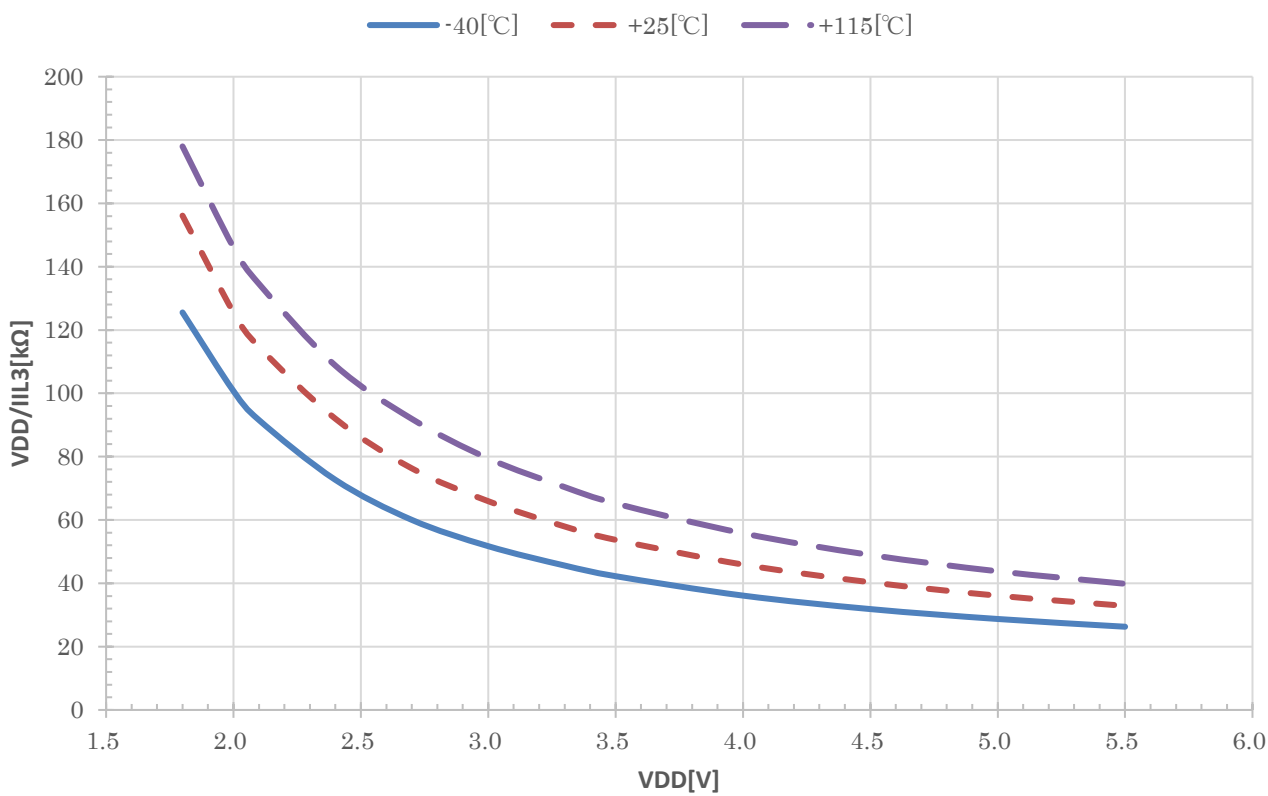
VDD vs VDD/IIL3 (TYP. VIL=VSS)
