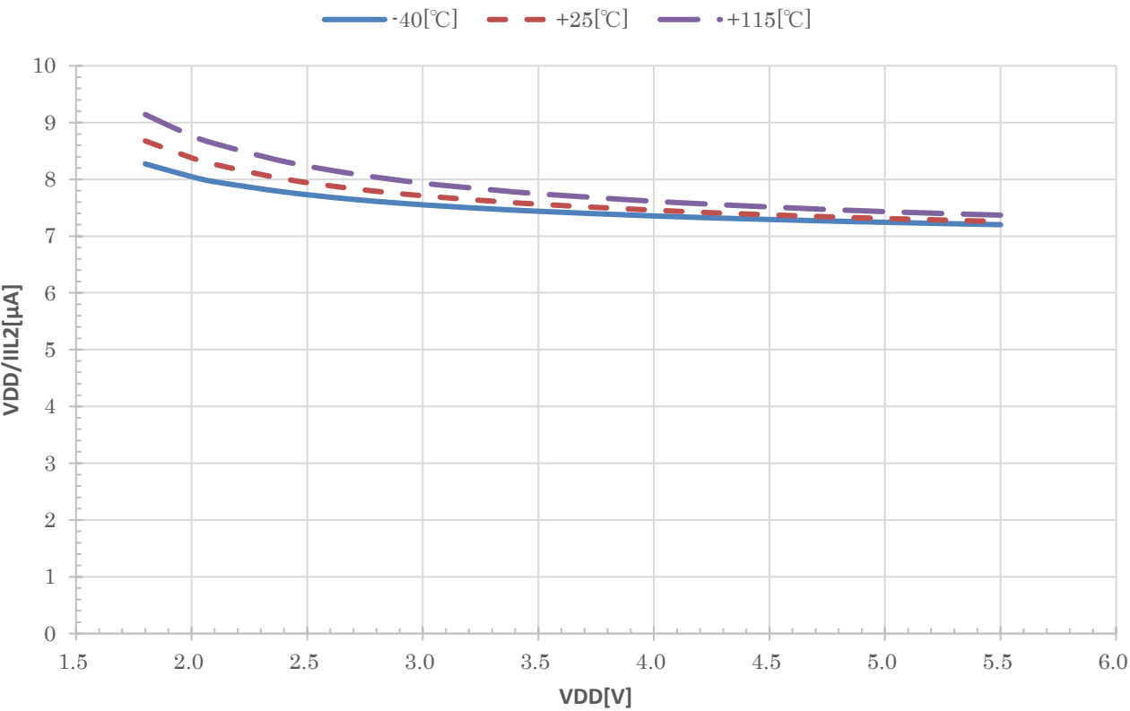
VDD/IIL2 vs VDD (TYP. VIL=VSS)
