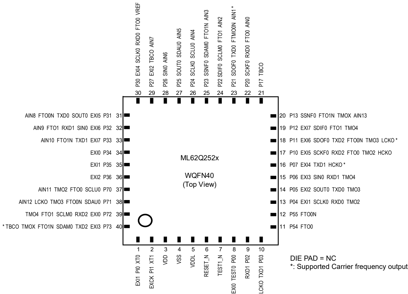
Fig.3-3 40 pin WQFN
