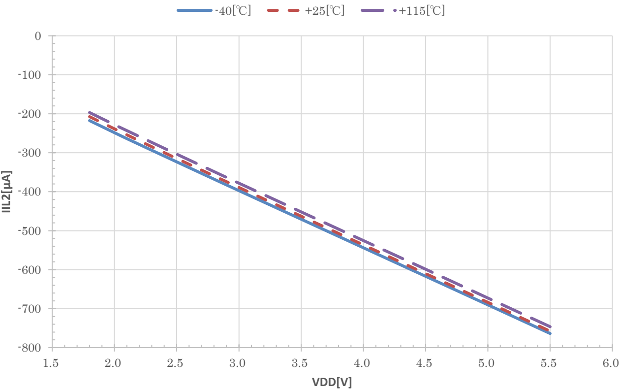
IIL2 vs VDD (TYP. VIL=VSS)
