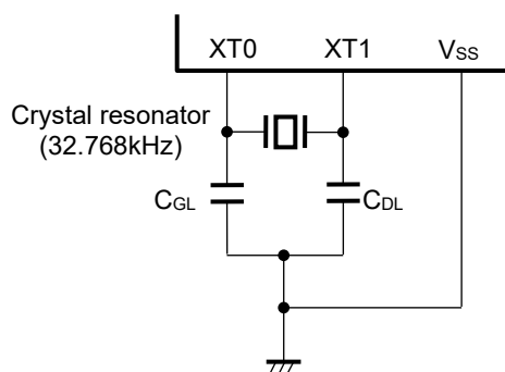
Example of external circuit for Low speed Crystal Oscillation
