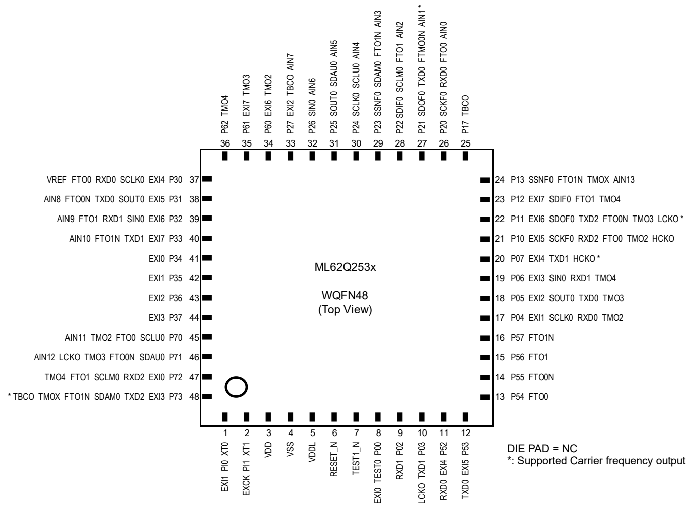
Fig.3-2 48 pin WQFN
