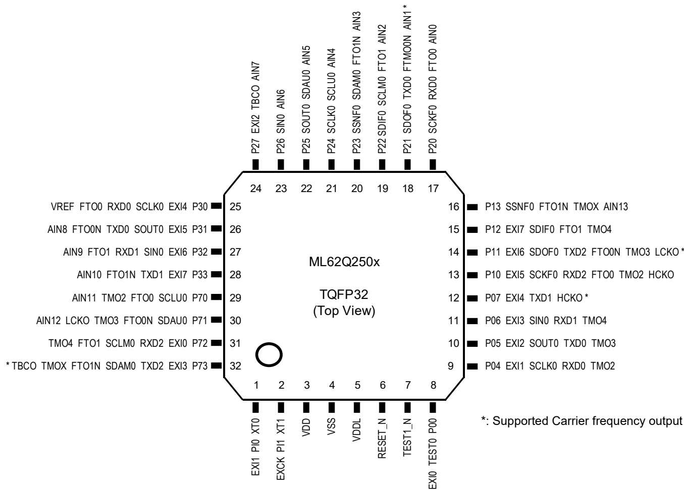
Fig.3-4 32 pin TQFP
