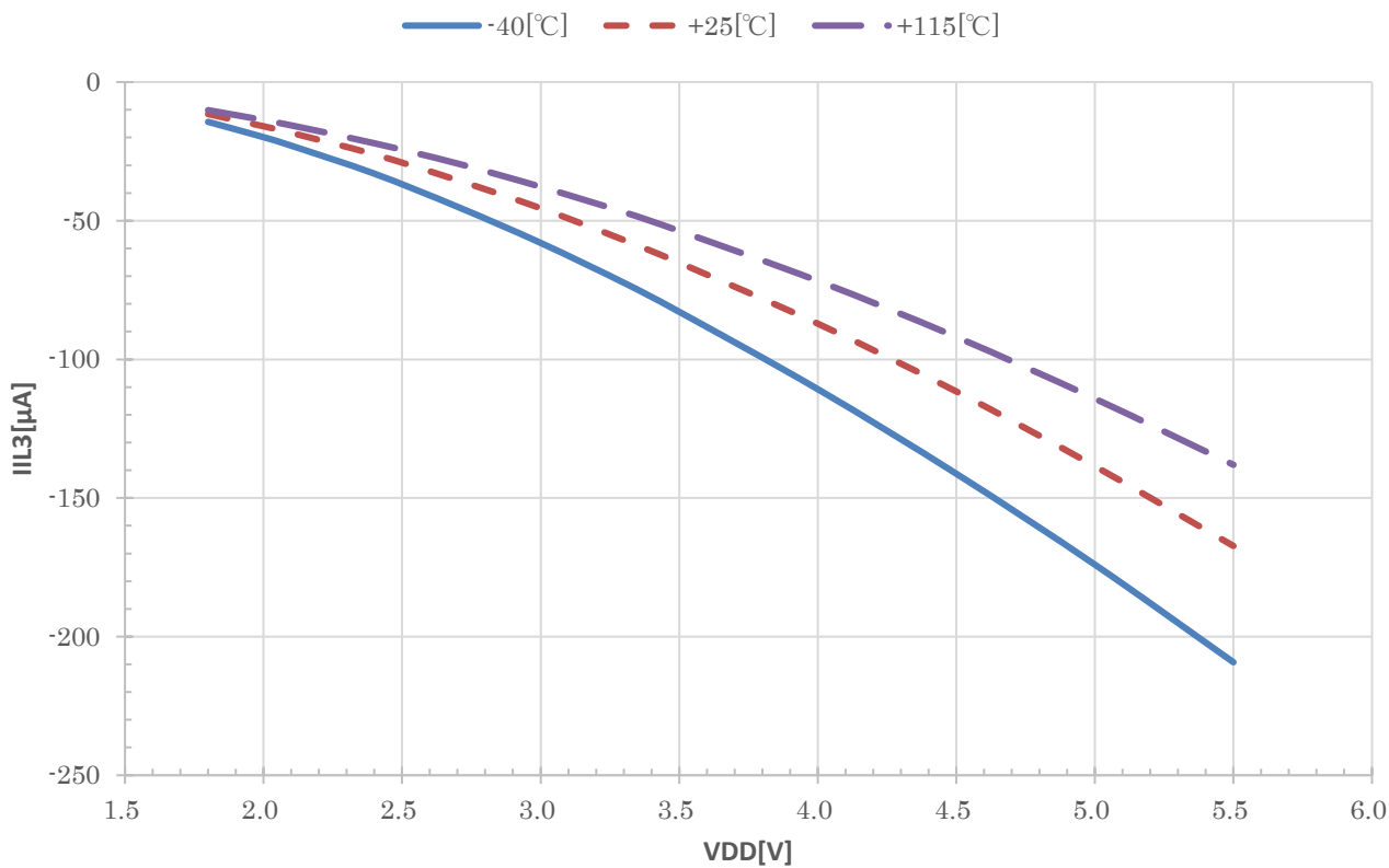
IIL3 vs VDD (TYP. VIL=VSS)
