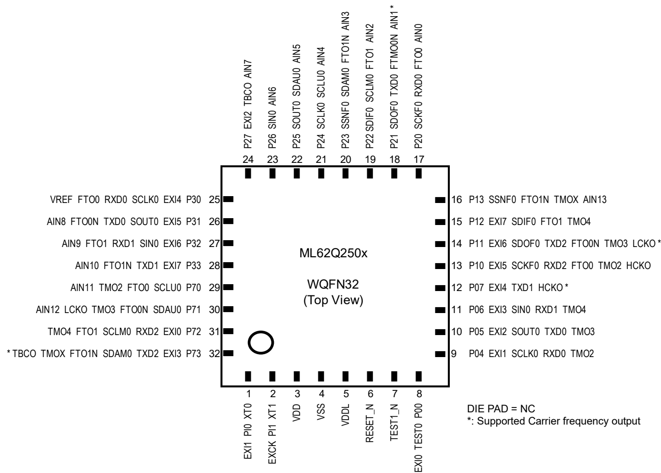
Fig.3-5 32 pin WQFN
