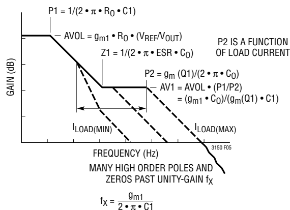
Figure 5. Typical Bode Plot for Tantalum or Electrolytic Output Capacitors
