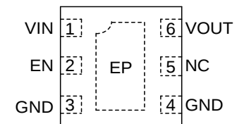
U-DFN2020-6 (SWP) (Type UXC)
