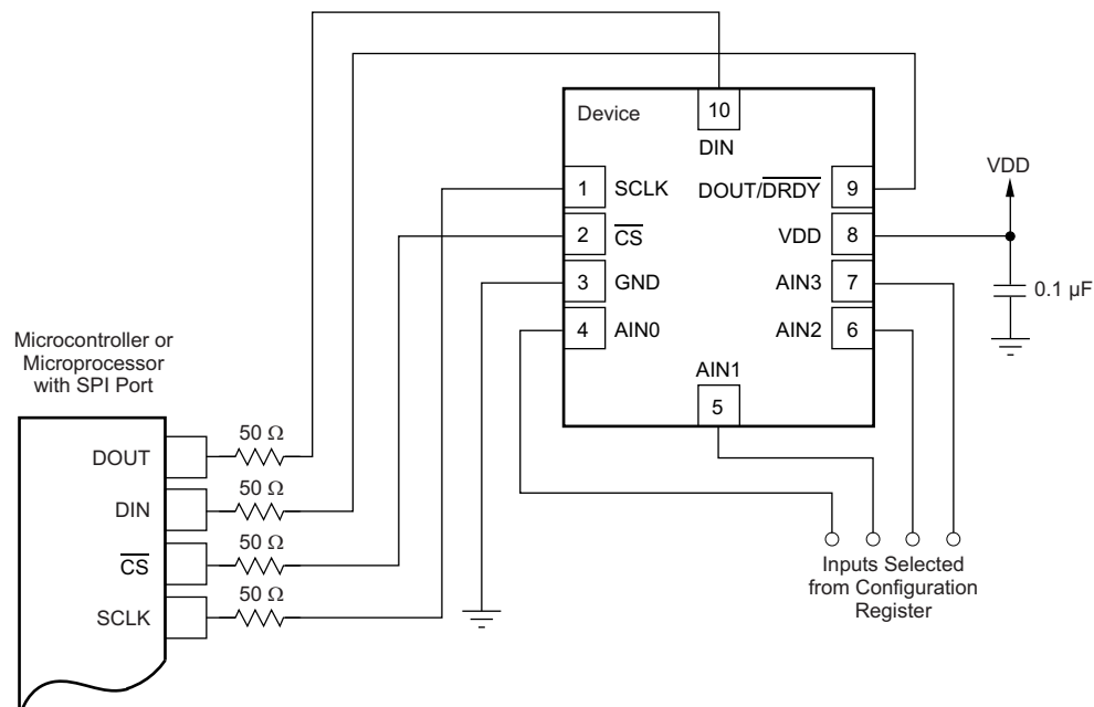
Figure 39. Typical Connections
