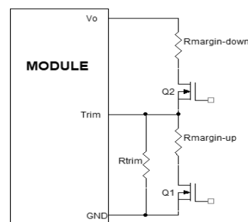
Figure 37. Circuit Configuration for margining Output voltage
