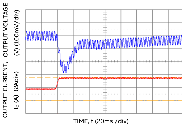
Figure 16. Transient Response to Dynamic Load Change from 50% to 100% at 28Vin, Cext - 3x10uF ceramic CTune=470pF & RTune=150Ω
