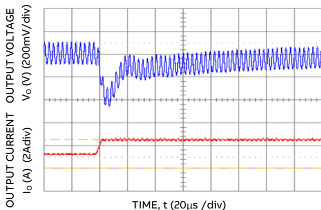
Figure 22. Transient Response to Dynamic Load Change from 50% to 100% at 28Vin, Cext = 1x10μF ceramic, CTune=150pF & RTune=220Ω
