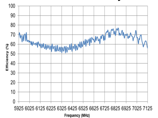
6 / 7 GHz Efficiency
