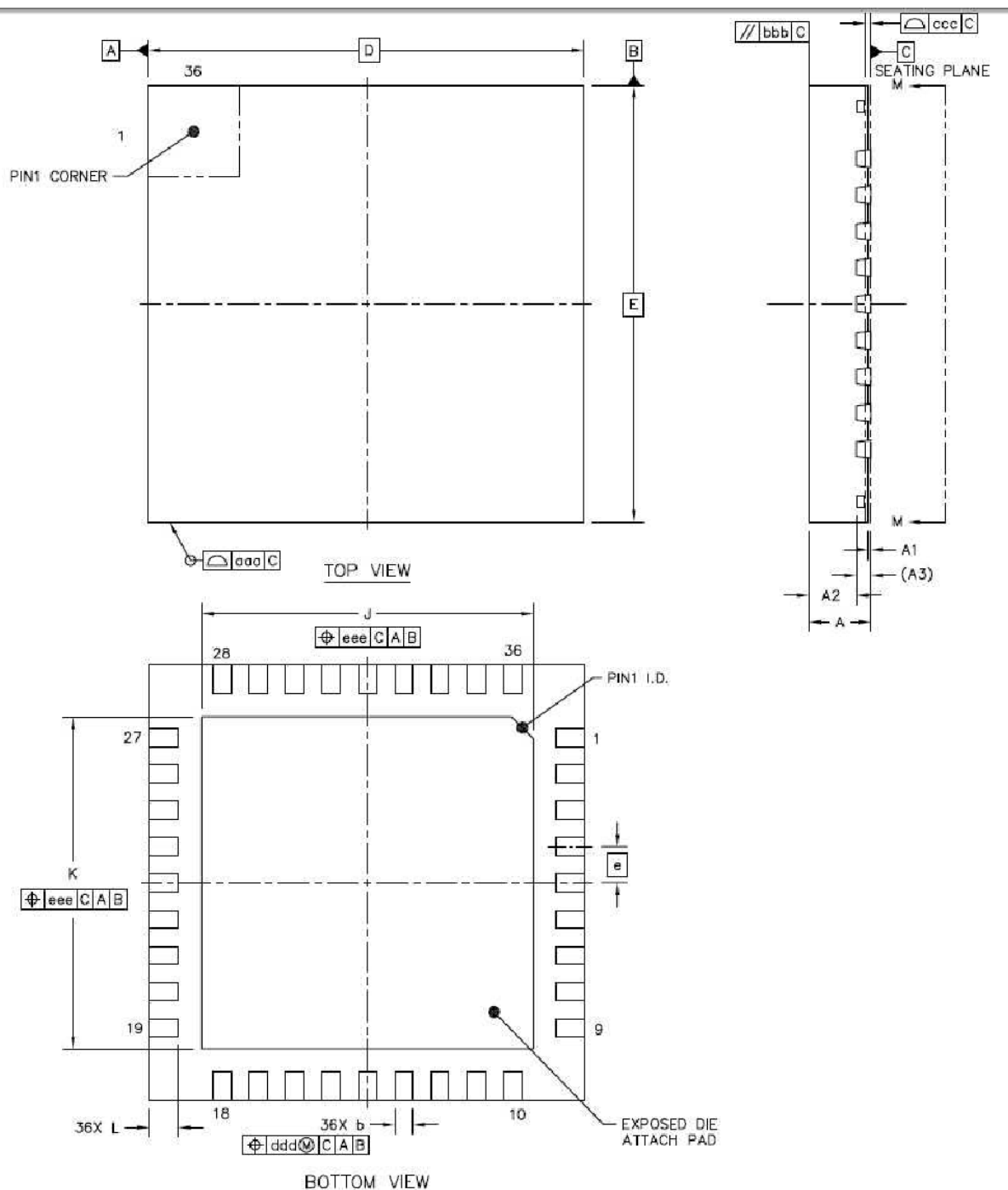
Figure 19. QFN36 pin 6x6
