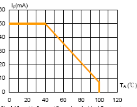
Fig. 4 Allowable Forward Current vs. Ambient Temperature
