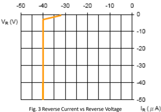
Fig. 3 Reverse Current vs Reverse Voltage
