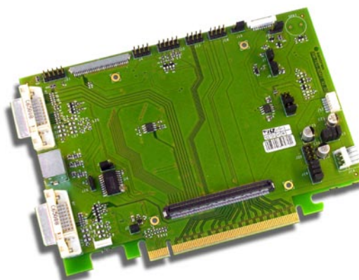
Optional PEG-Adapter board
