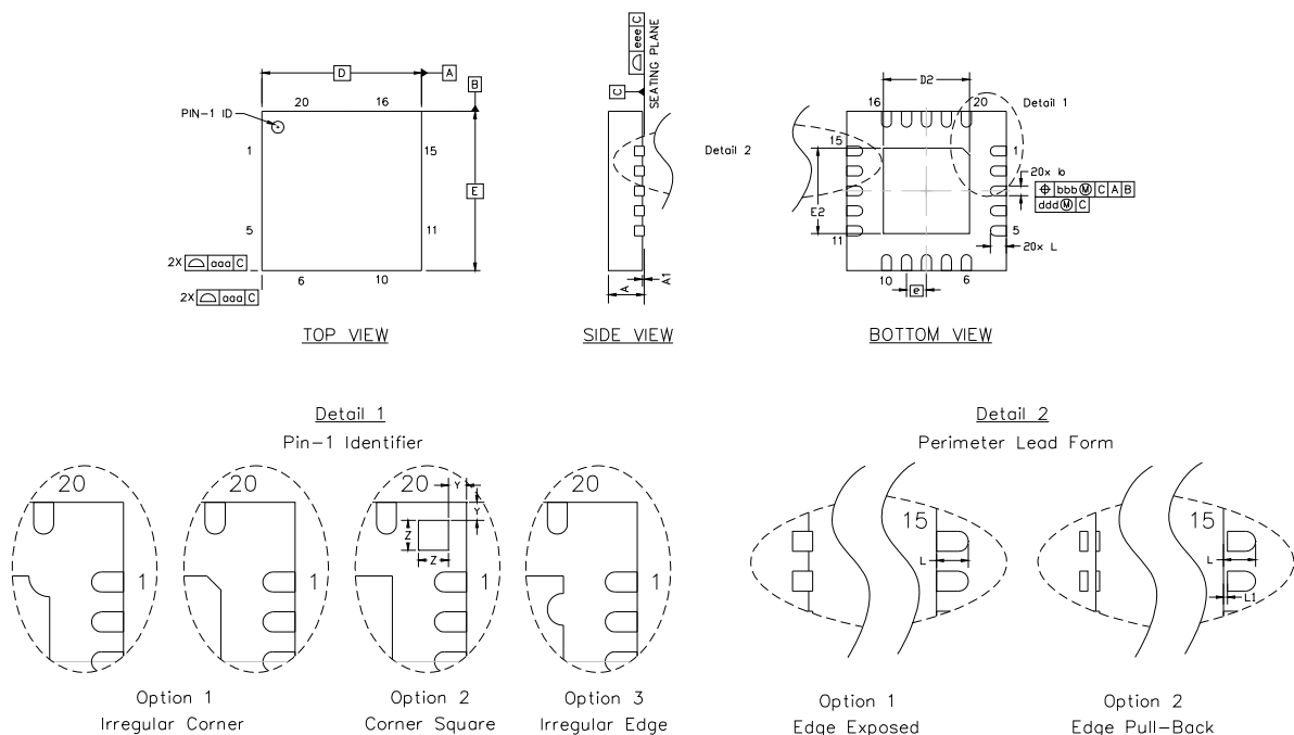
Figure 2. QFN-20 Package Drawing
