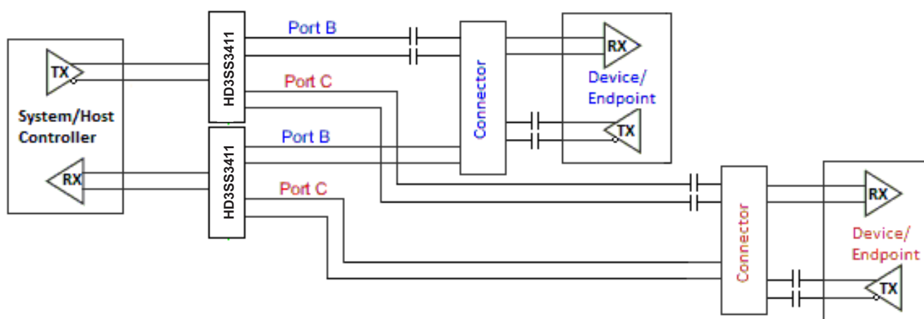
Figure 4. AC Coupling Capacitors Between Switch TX and Endpoint TX
