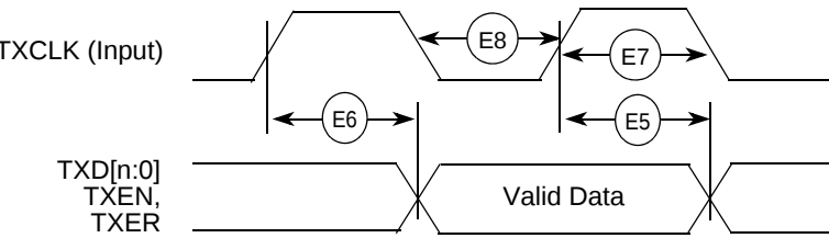
Figure 20. MII Transmit Signal Timing Diagram
