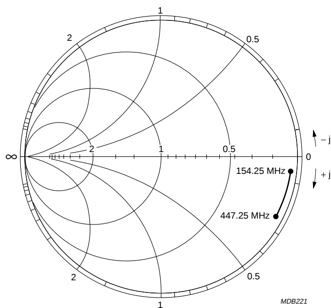
Fig.6 Input admittance ( S_{11} ) of the MID band mixer (154.25 to 447.25 MHz); Y_O = 10 mS.
