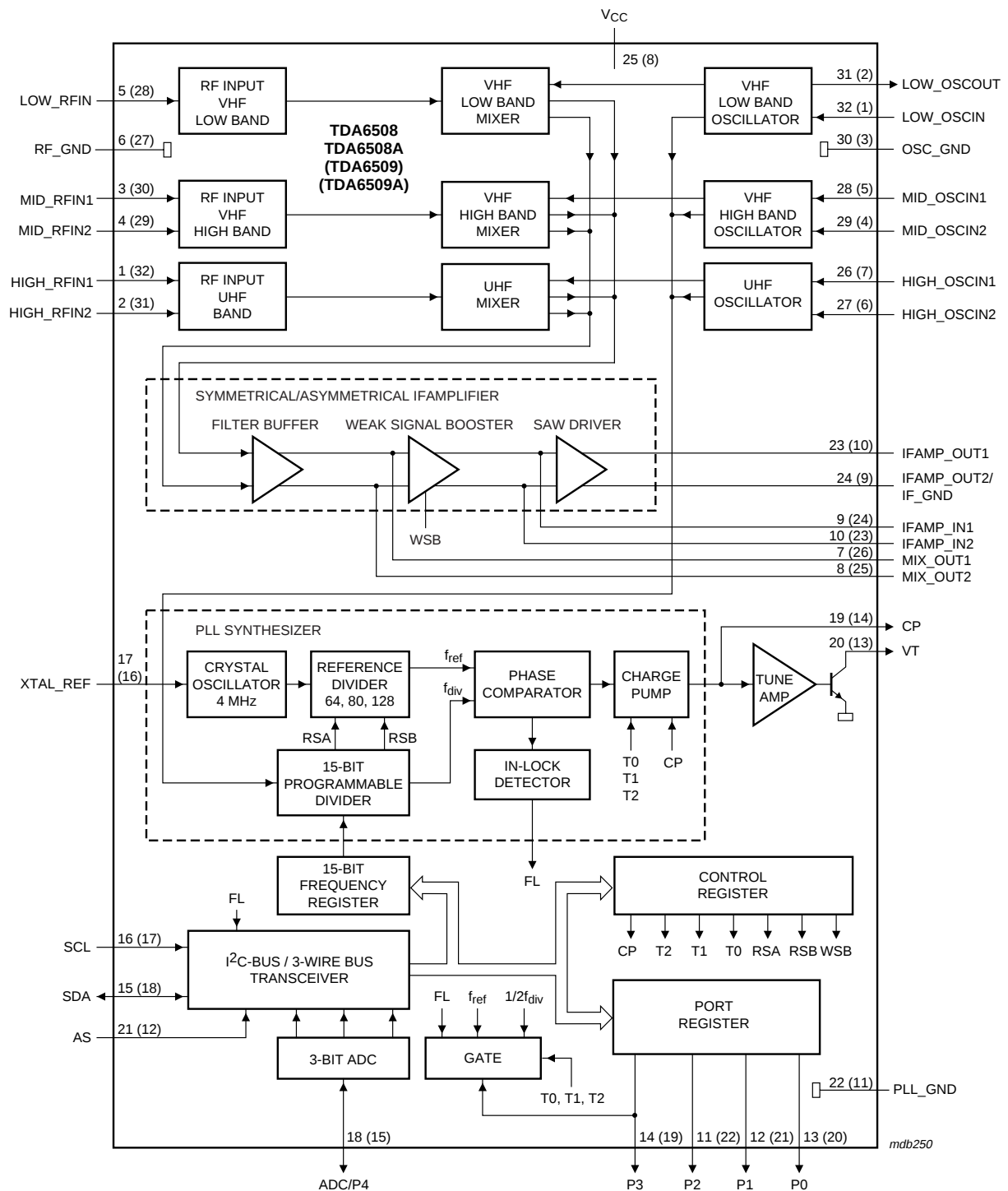
Fig.1 Block diagram.
