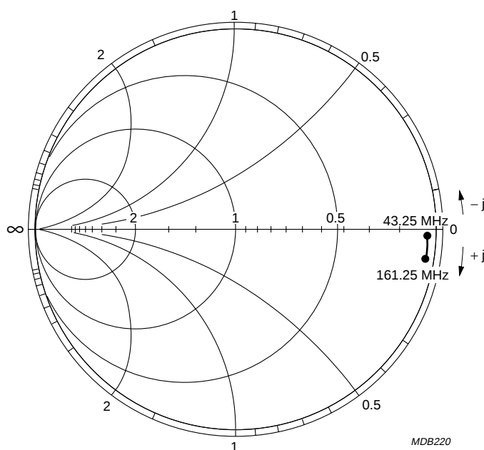
Fig.5 Input admittance ( S_{11} ) of the LOW band mixer (43.25 to 161.25 MHz); Y_O = 20 mS.
