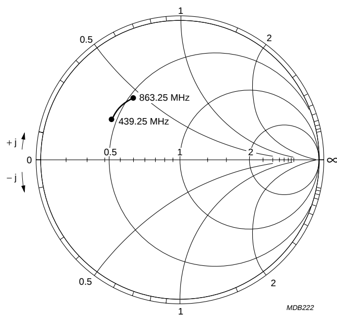
Fig.7 Input impedance ( S_{11} ) of the HIGH band mixer (439.25 to 863.25 MHz); Z_0 = 100 \Omega .
