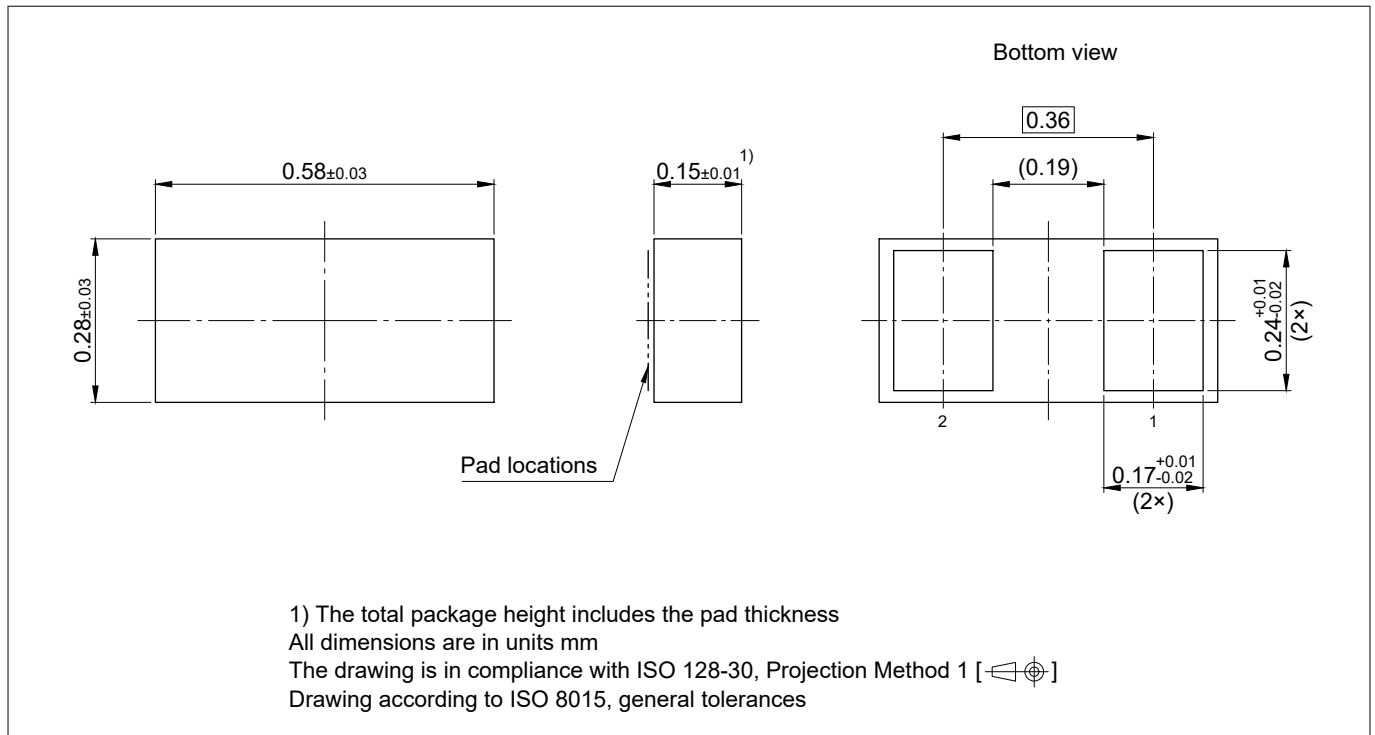
Figure 11 WLL-2-3 package
