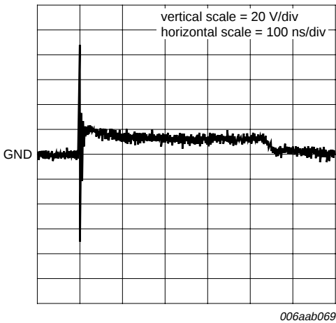
Fig 18. PESD5Z12: Clamped +8 kV ESD pulse waveform (IEC 61000-4-2 network)
