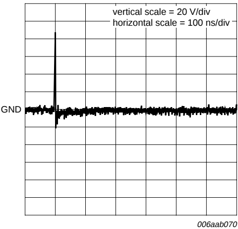
Fig 19. PESD5Z12: Clamped -8 kV ESD pulse waveform (IEC 61000-4-2 network)
