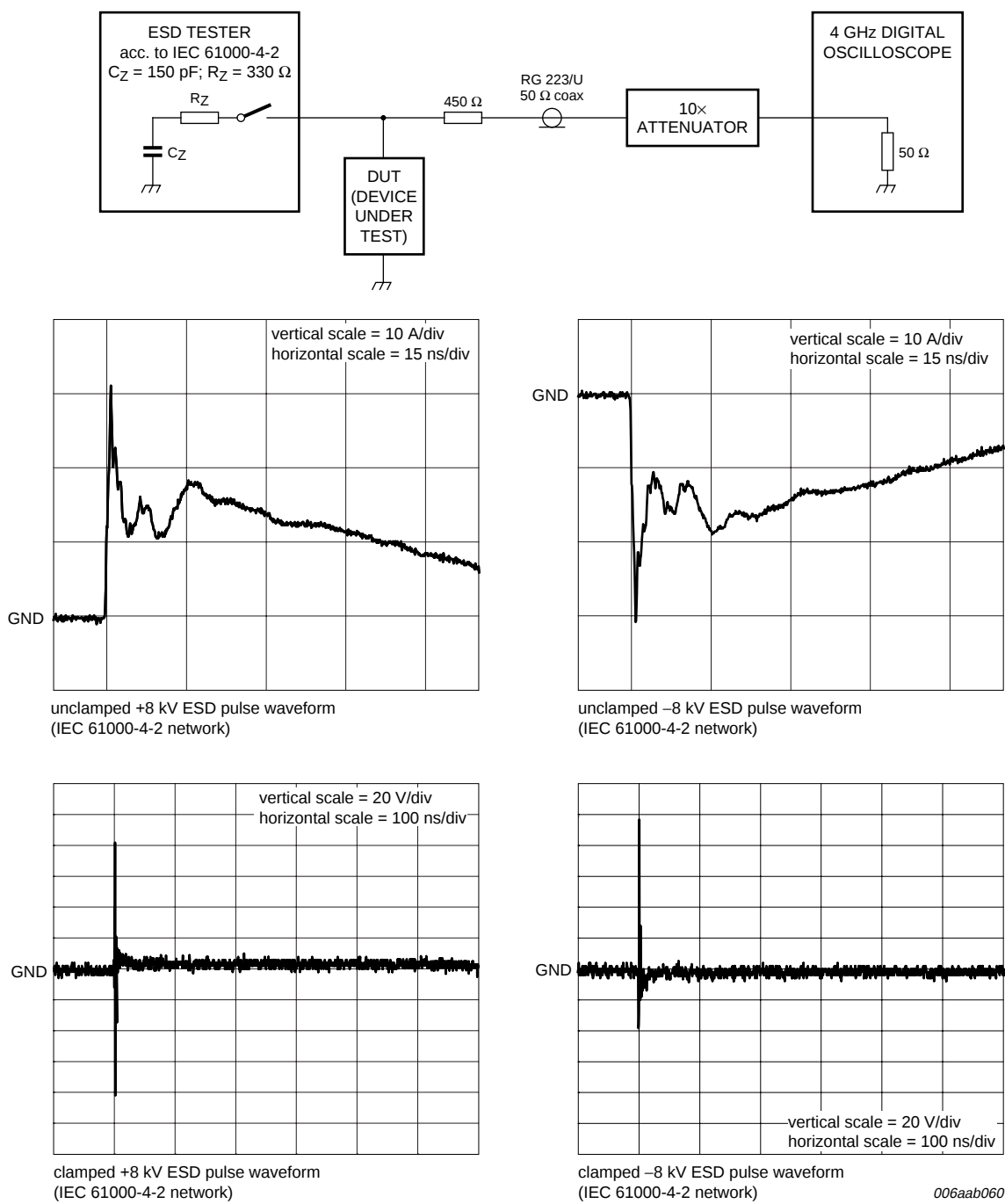
Fig 9. ESD clamping test setup and waveforms for PESD5Z2.5
