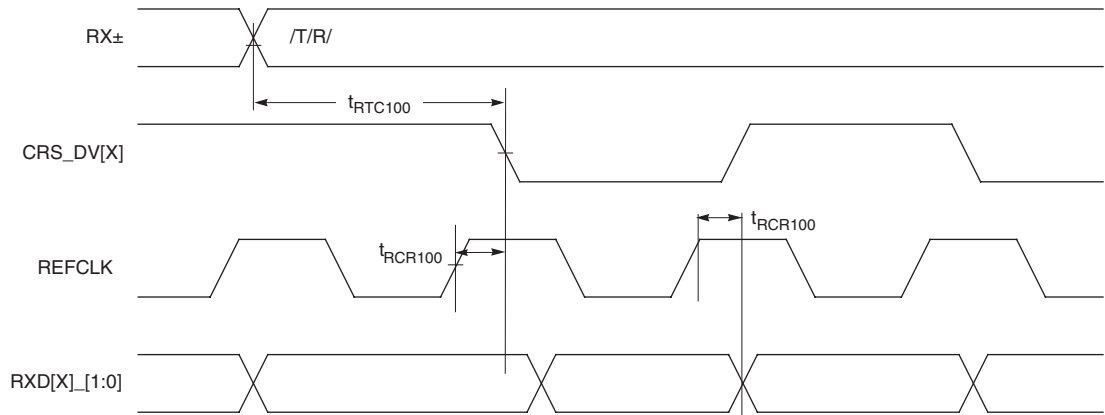
Figure 23. 100 Mbps RMII Receive End of Packet Timing
