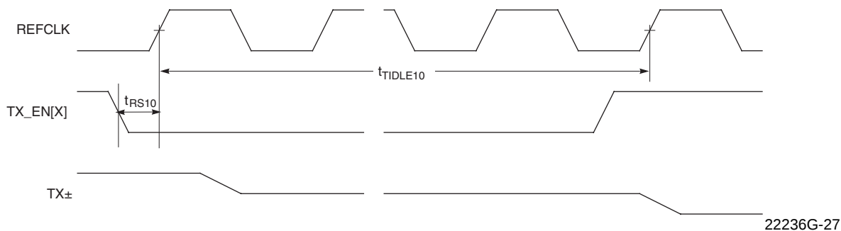
Figure 25. RMII 10 Mbps Transmit End of Packet Timing
