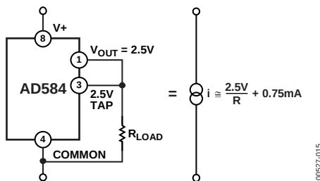
Figure 14. A Two-Component Precision Current Limiter
