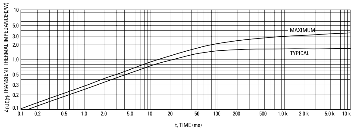
Figure 10. Thermal Response
