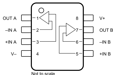
OPA2320-Q1: DGK Package 8-Pin VSSOP Top View
