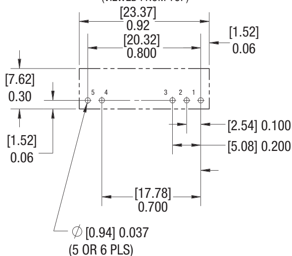
RECOMMENDED FOOTPRINT (VIEWED FROM TOP)
