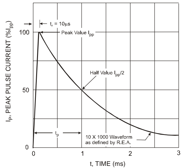
Figure 4. Pulse Waveform
