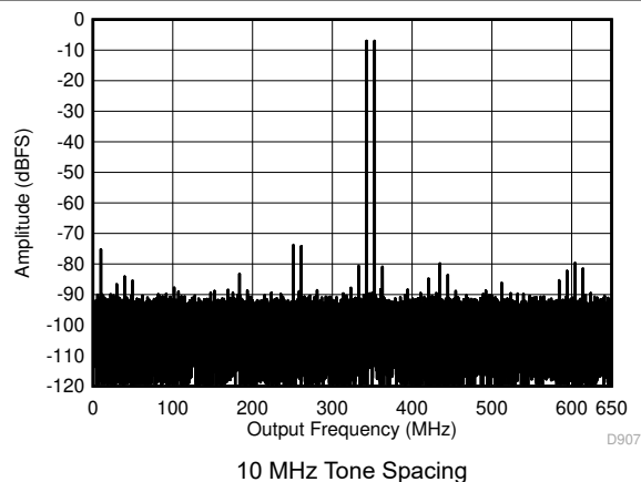
Figure 7-49. Two Tone FFT at 348 MHz Center
