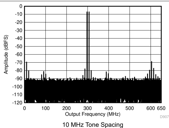
Figure 7-51. Two Tone FFT at 998 MHz Center
