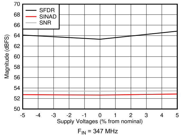
Figure 7-44. SNR, SFDR and SINAD vs Supply Voltage
