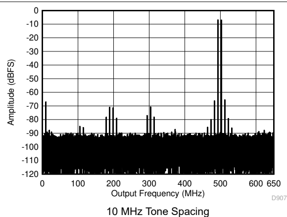
Figure 7-52. Two Tone FFT at 1798 MHz Center
