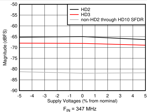
Figure 7-45. HD2, HD3 and Worst non-HD Spur vs Supply Voltage
