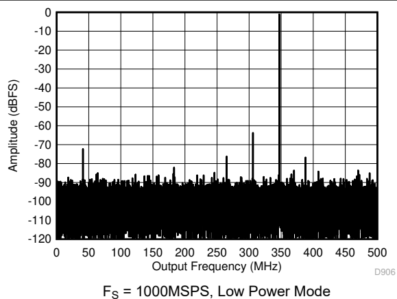
Figure 7-12. Single Tone FFT at 347 MHz and -1 dBFS
