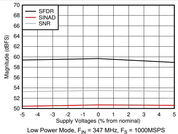
Figure 7-46. SNR, SFDR and SINAD vs Supply Voltage
