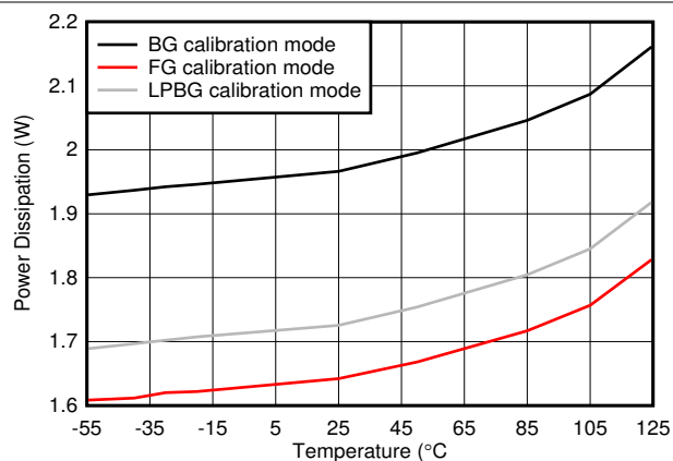
Figure 7-124. Dual Channel, Power Dissipation vs Temperature
