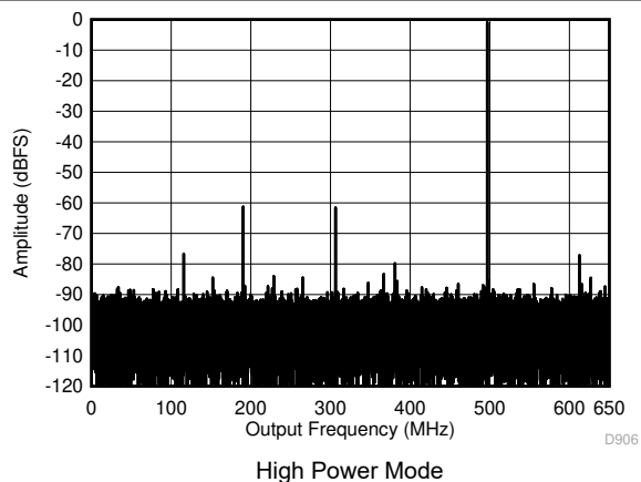
Figure 7-8. Single Tone FFT at 1797 MHz and -1 dBFS
