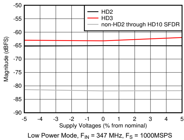
Figure 7-47. HD2, HD3 and Worst non-HD Spur vs Supply Voltage
