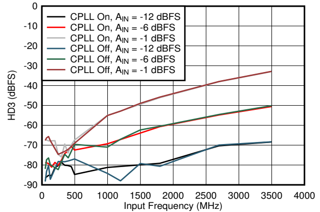
Figure 7-80. HD3 vs Input Frequency, CPLL and Input Amplitude
