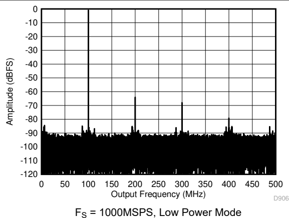
Figure 7-11. Single Tone FFT at 99.997 MHz and -1 dBFS
