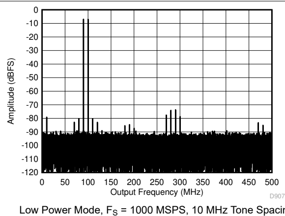
Figure 7-54. Two Tone FFT at 95.07 MHz Center
