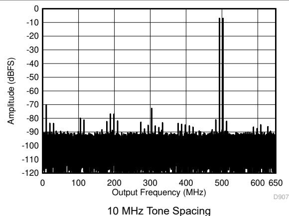
Figure 7-50. Two Tone FFT at 498 MHz Center
