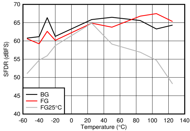
Figure 7-43. SFDR vs Temperature and Calibration Mode
