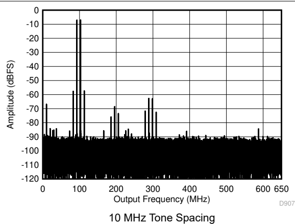
Figure 7-53. Two Tone FFT at 2698 MHz Center
