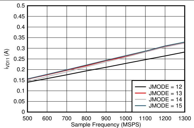
Figure 7-100. Dual Channel, I_{VD11} vs FS and JMODE 12 - 15
