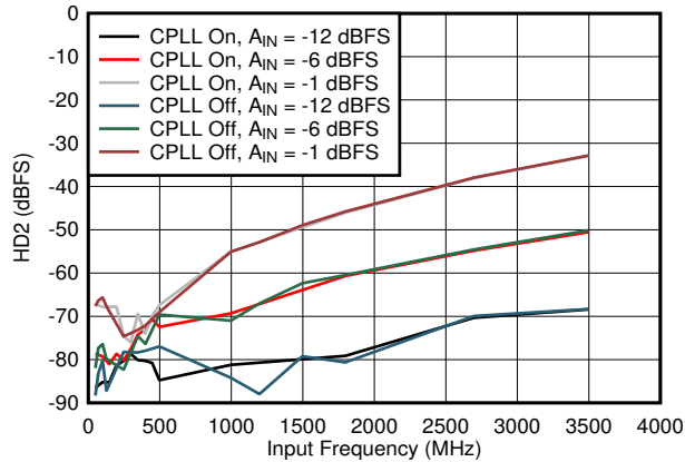
Figure 7-79. HD2 vs Input Frequency, CPLL and Input Amplitude
