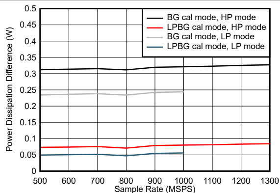
Figure 7-111. Quad Channel, Power Dissipation Change with Calibration Mode
