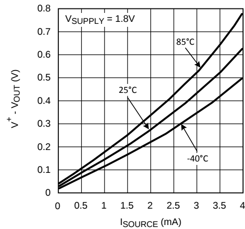
Figure 10. Output Positive Swing vs. I_{\text{SOURCE}}
