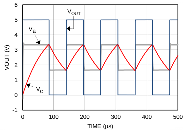
Figure 37. Square Wave Oscillator Output Waveforms
