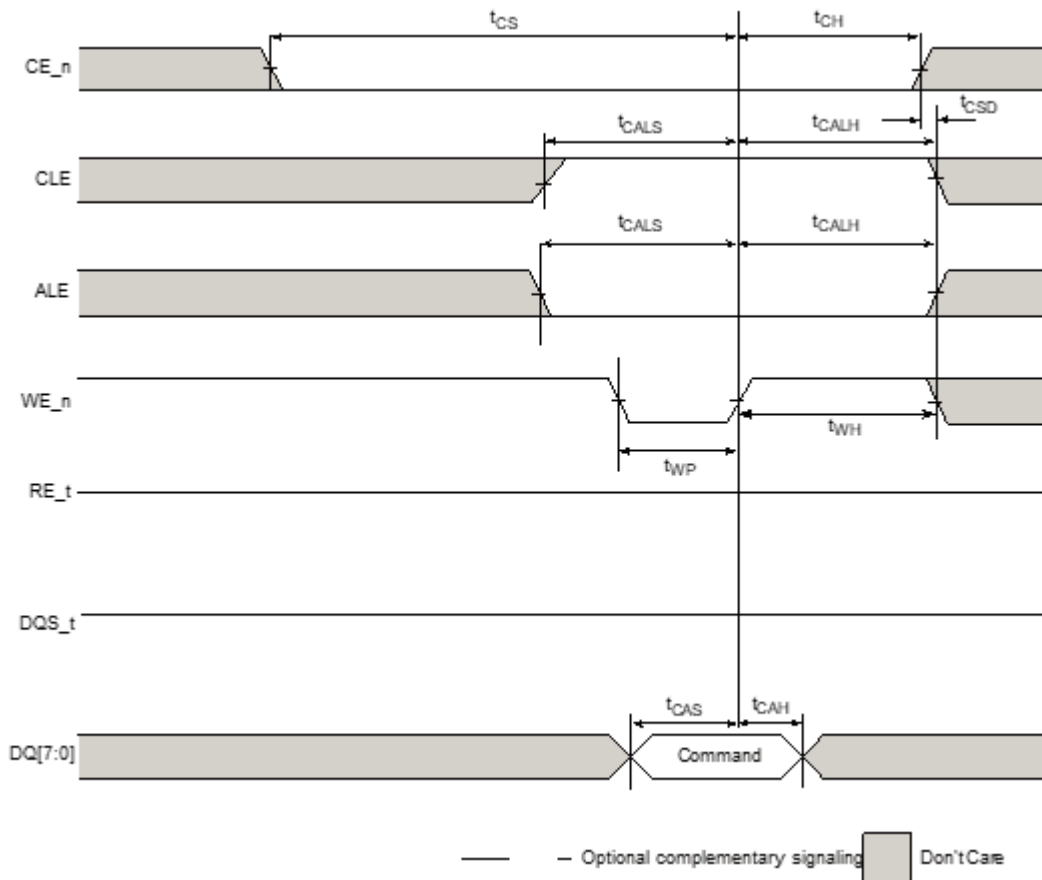
Figure 35. Command cycle
