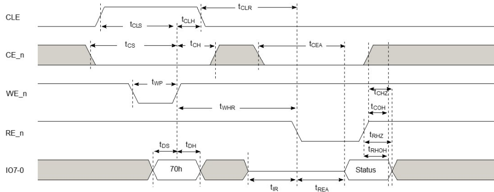
Figure 40. Read status timings
