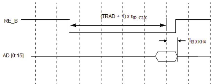
Figure 47. t_{BIXKH4} timings
