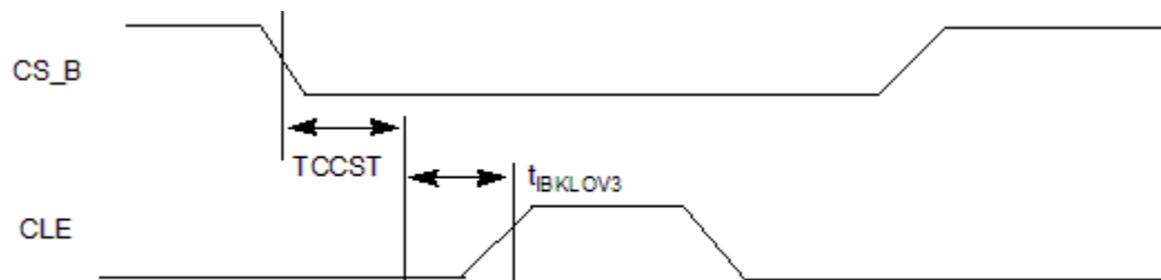
Figure 33. IFC-NAND interface output AC timings
