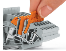
Jumper with safety lid Removing a jumper via safety lid.
